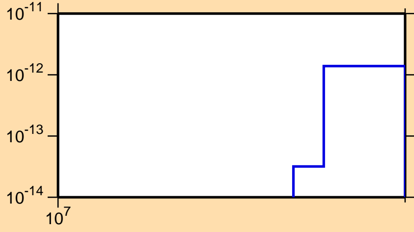
\sigma vs. E for ^{136}\text{La} (mt 45)
