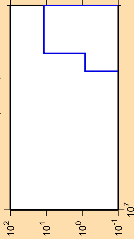
\Delta\sigma/\sigma vs. E for ^{136}\text{La}(\text{mt117})
