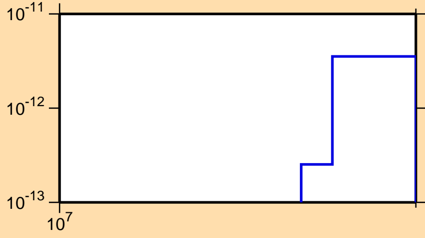
\sigma vs. E for ^{136}\text{La}(\text{mt117})
