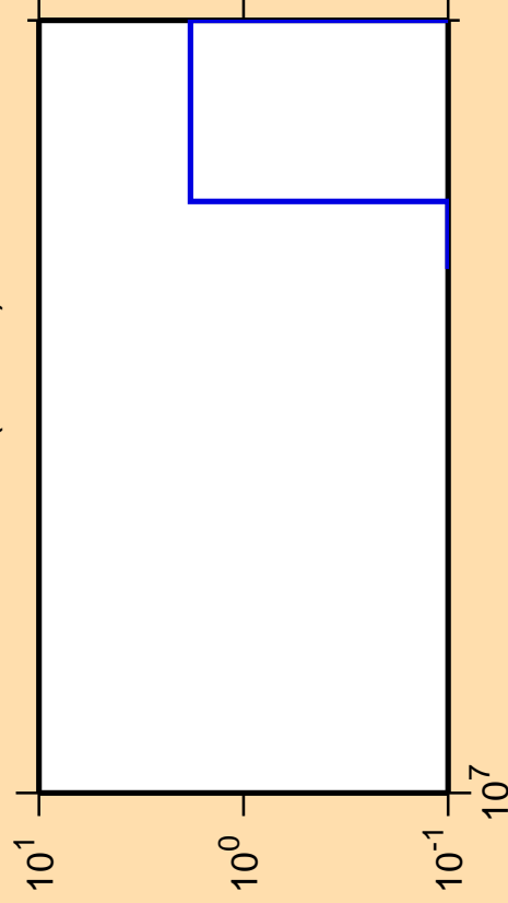
\Delta\sigma/\sigma vs. E for ^{136}\text{La} (mt 45)
