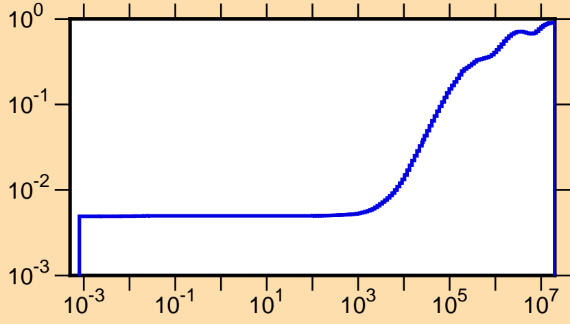
\mu vs. E for ^{137}\text{La}(\text{mt251})
