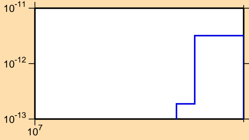
\sigma vs. E for ^{137}\text{La}(\text{mt117})
