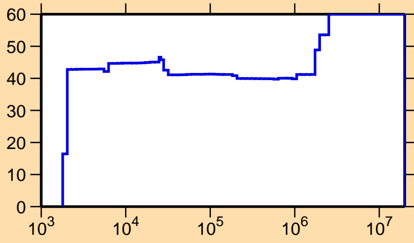
\Delta\sigma/\sigma vs. E for ^{137}\text{La}(n,\gamma)
