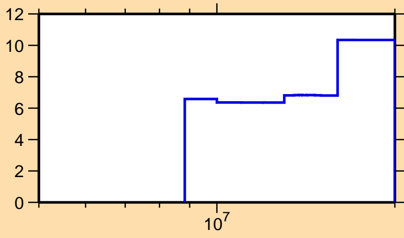
\Delta\sigma/\sigma vs. E for ^{137}\text{La}(n,\text{el.})
