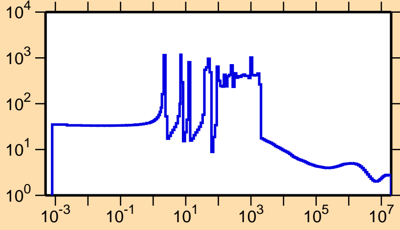
\sigma vs. E for ^{137}\text{La}(n,\text{el.})
