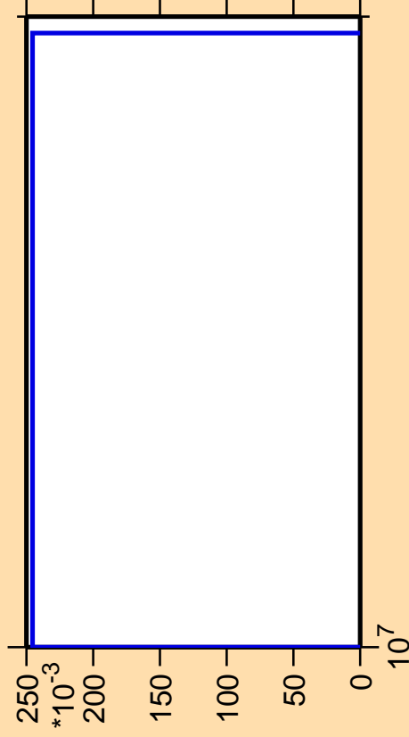
\Delta\sigma/\sigma vs. E for ^{137}\text{La}(\text{mt117})
