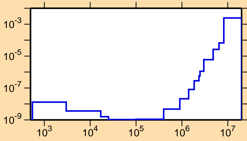
\sigma vs. E for ^{137}\text{La}(n,\alpha)
