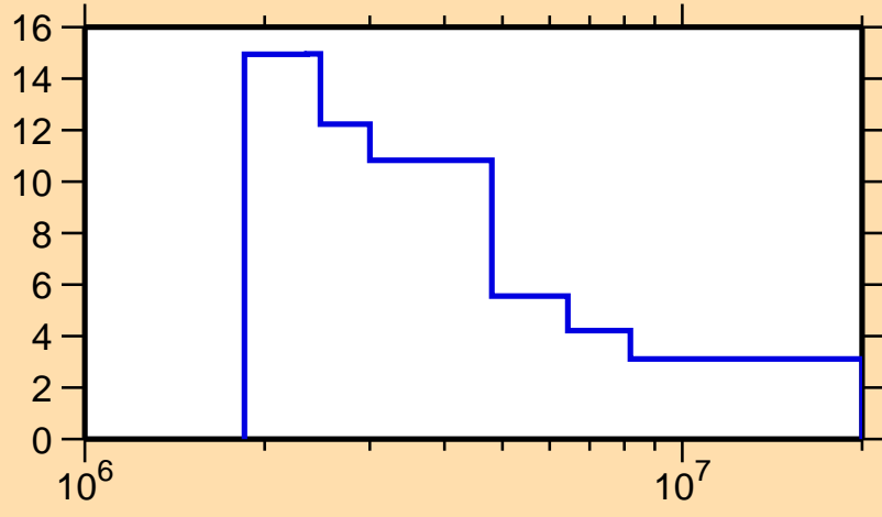
\Delta\sigma/\sigma vs. E for ^{137}\text{La}(n, \text{tot.})
