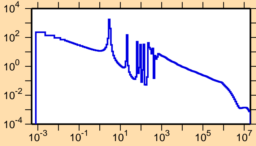
\sigma vs. E for ^{138}\text{La}(n,\gamma)
