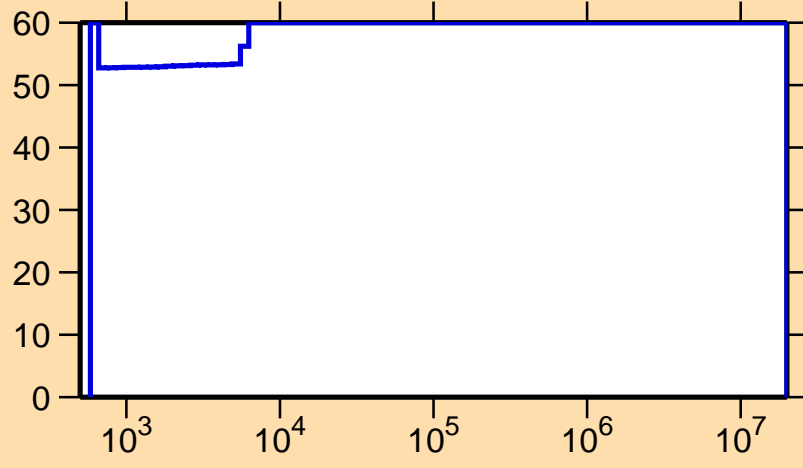
\Delta\sigma/\sigma vs. E for ^{138}\text{La}(n,\gamma)
