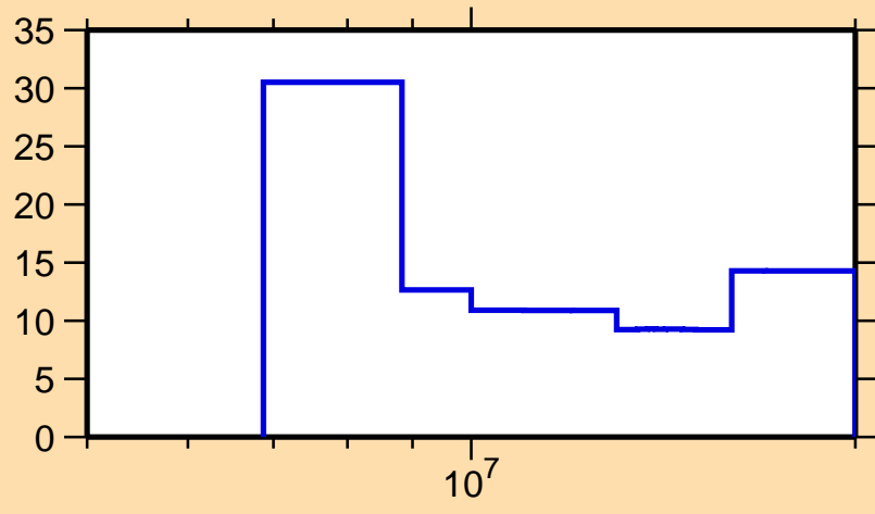
\Delta\sigma/\sigma vs. E for ^{138}\text{La}(n,2n)
