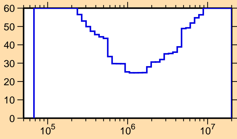
\Delta\sigma/\sigma vs. E for ^{138}\text{La}(n,n_1)
