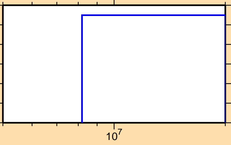
\sigma vs. E for ^{138}\text{La}(n,2n\alpha)
