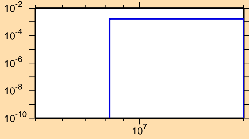
\sigma vs. E for ^{138}\text{La}(n,np)
