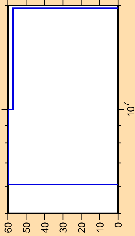
\Delta\sigma/\sigma vs. E for ^{139}\text{La}(n,np)
