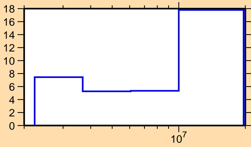
Delta \sigma/\sigma vs. E for ^{139}\text{La}(n,n\text{cont.})
