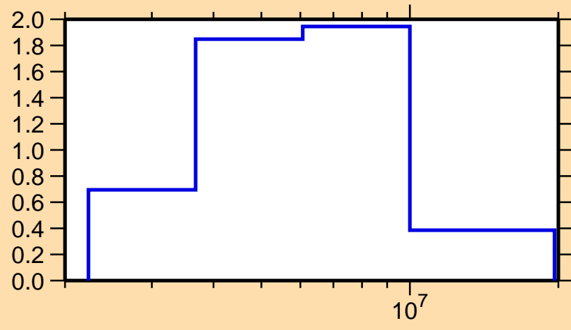
\sigma vs. E for ^{139}\text{La}(n,n\text{cont.})
