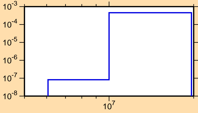
\sigma vs. E for ^{139}\text{La}(n,np)
