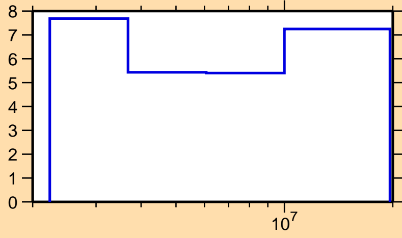
\Delta\sigma/\sigma vs. E for ^{139}\text{La}(n, n_{\text{nonel}})
