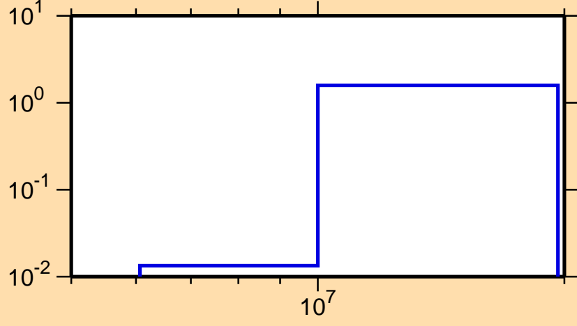
\sigma vs. E for ^{139}\text{La}(n,2n)
