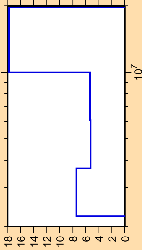
\Delta\sigma/\sigma vs. E for ^{139}\text{La}(n,n\text{cont.})
