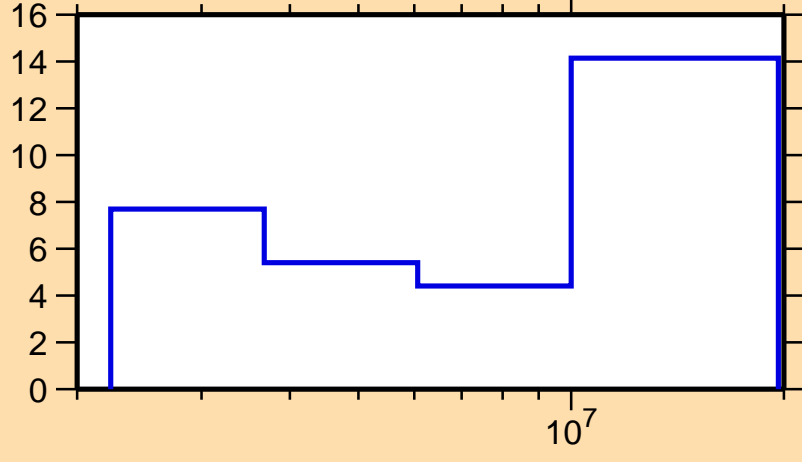
Δσ/σ vs. E for ^{139}\text{La}(n,\text{inel.})
