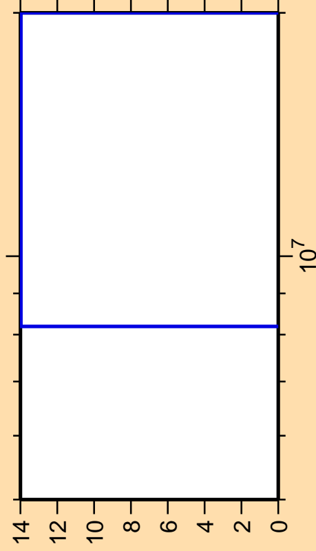
\Delta\sigma/\sigma vs. E for ^{139}\text{La}(n,n\text{cont.})
