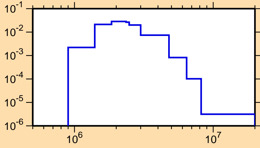
\sigma vs. E for ^{139}\text{La}(n,n_2)
