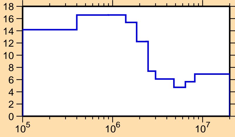
\Delta\sigma/\sigma vs. E for ^{139}\text{La}(n,\text{nonel.})
