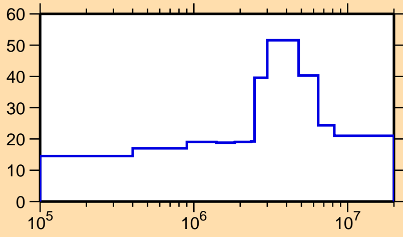
\Delta\sigma/\sigma vs. E for ^{139}\text{La}(n,n_1)
