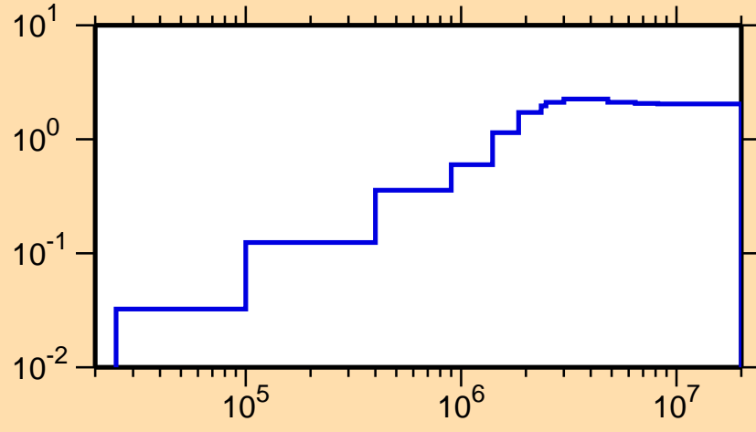
\sigma vs. E for ^{139}\text{La}(n,\text{nonel.})
