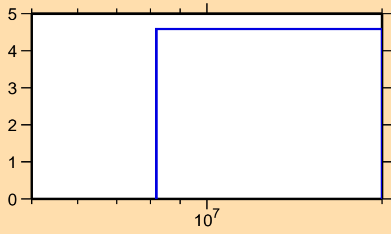
\Delta\sigma/\sigma vs. E for ^{139}\text{La}(n,\text{tot.})
