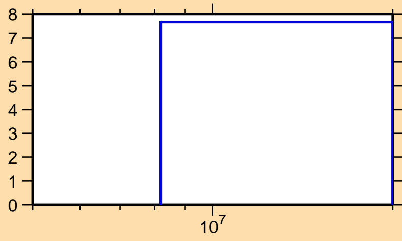
\Delta\sigma/\sigma vs. E for ^{139}\text{La}(n,\text{el.})
