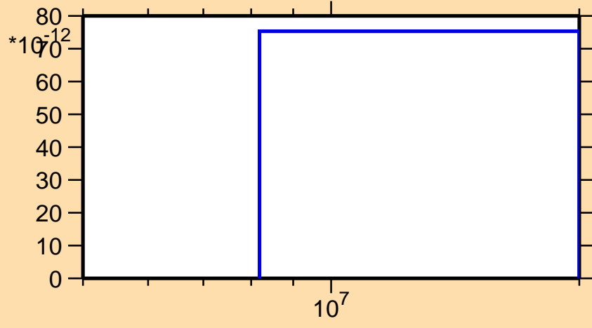
\sigma vs. E for ^{139}\text{La}(n,\text{He3})
