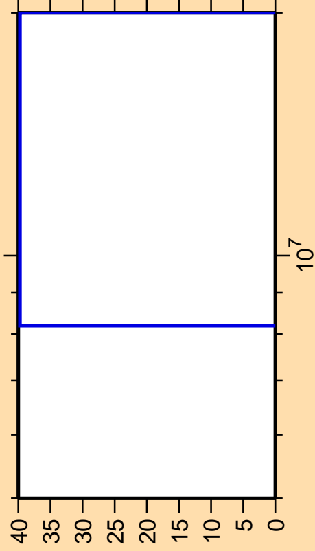
\Delta\sigma/\sigma vs. E for ^{139}\text{La}(n,2n\alpha)
