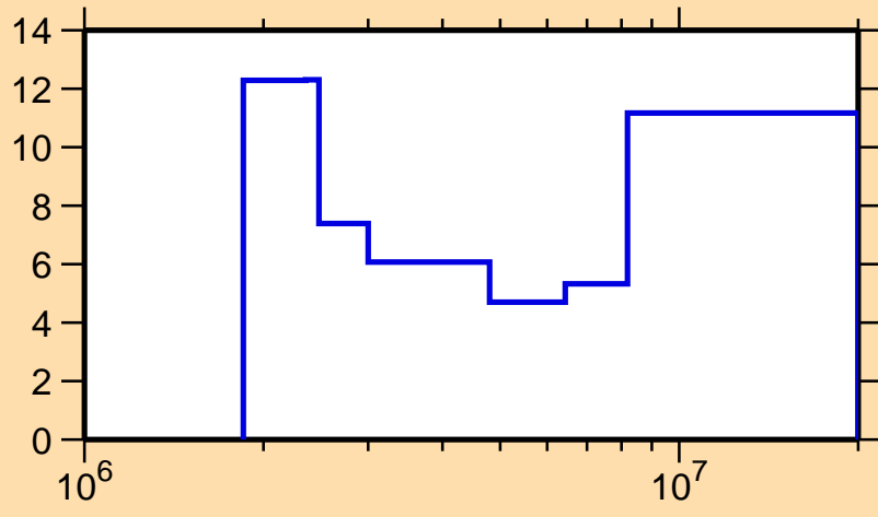
\Delta\sigma/\sigma vs. E for ^{139}\text{La}(n,\text{inel.})
