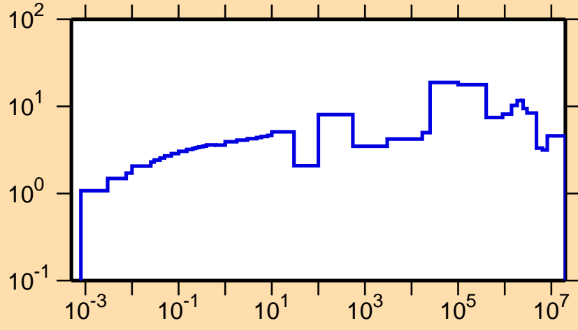
\Delta\sigma/\sigma vs. E for ^{139}\text{La}(n,\text{tot.})
