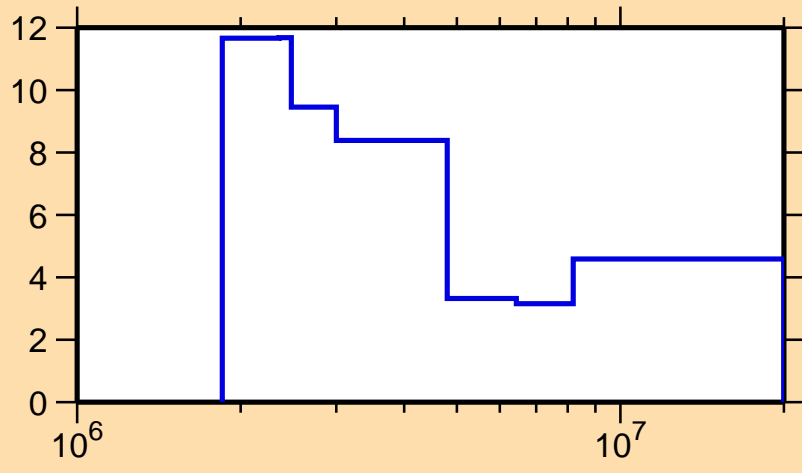
\Delta\sigma/\sigma vs. E for ^{139}\text{La}(n,\text{tot.})
