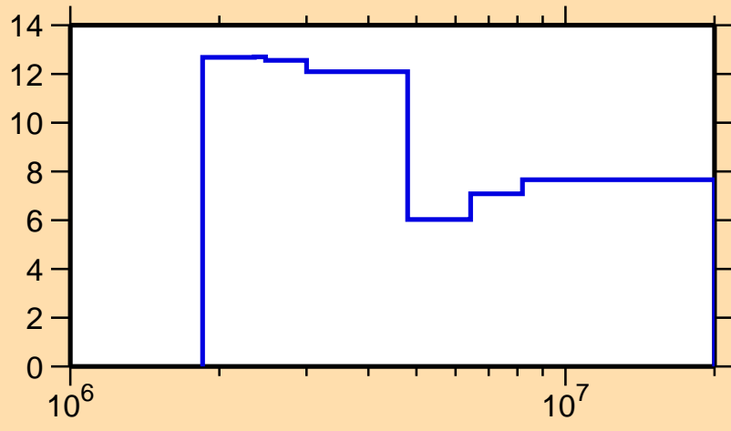
\Delta\sigma/\sigma vs. E for ^{139}\text{La}(n,\text{el.})
