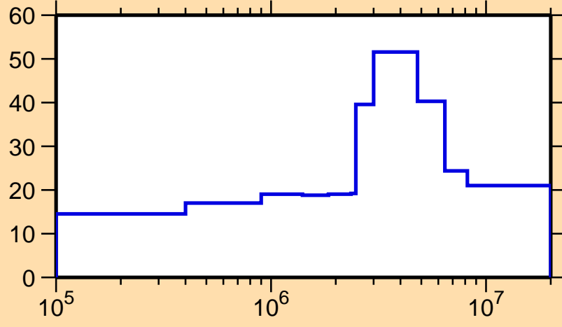
\Delta\sigma/\sigma vs. E for ^{139}\text{La}(n,n_1)
