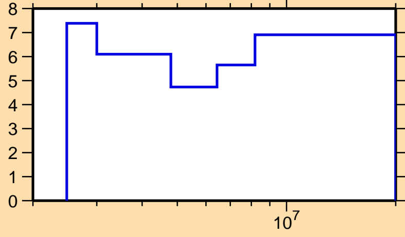
\Delta\sigma/\sigma vs. E for ^{139}\text{La}(n,\text{nonel.})
