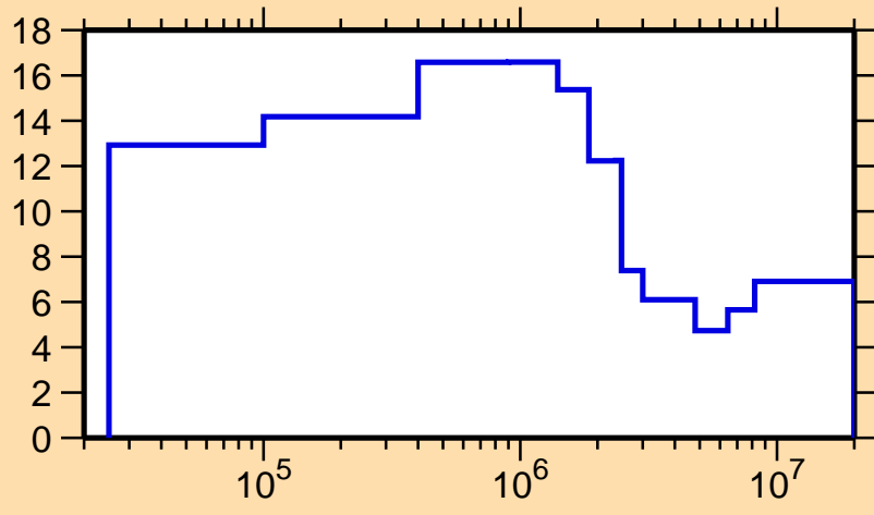
\Delta\sigma/\sigma vs. E for ^{139}\text{La}(n,\text{nonel.})
