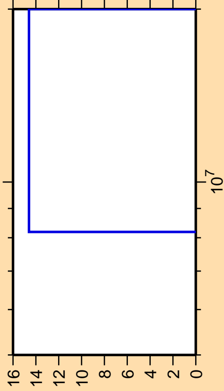
\Delta\sigma/\sigma vs. E for ^{139}\text{La}(n,\alpha)
