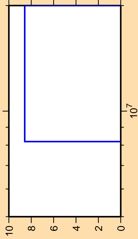
\Delta\sigma/\sigma vs. E for ^{139}\text{La}(n,p\alpha)
