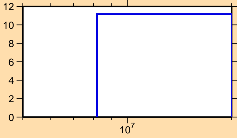
\Delta\sigma/\sigma vs. E for ^{139}\text{La}(n,\text{inel.})
