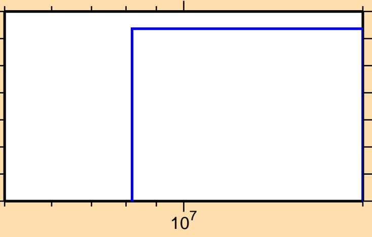
\sigma vs. E for ^{139}\text{La}(n,\text{nd})
