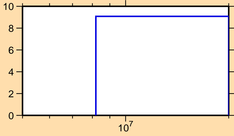
\Delta\sigma/\sigma vs. E for ^{139}\text{La}(n,2n)
