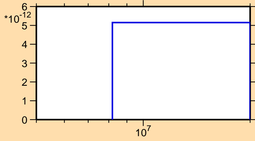
\sigma vs. E for ^{139}\text{La}(n,p\alpha)
