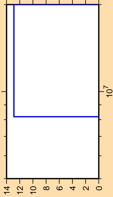
\Delta\sigma/\sigma vs. E for ^{139}\text{La}(n,p)
