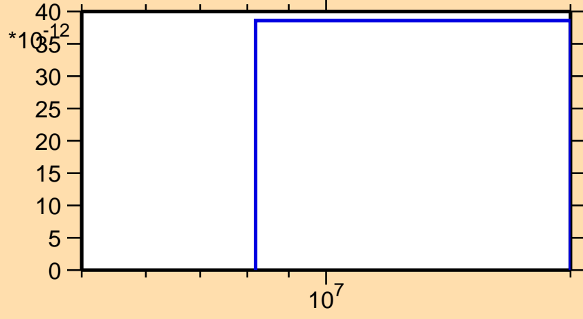
\sigma vs. E for ^{139}\text{La}(n,2n\alpha)
