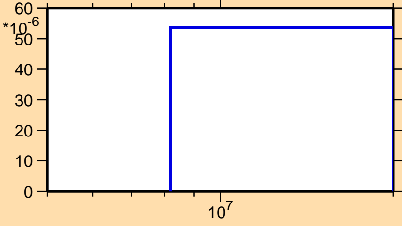
\sigma vs. E for ^{139}\text{La}(n,t)
