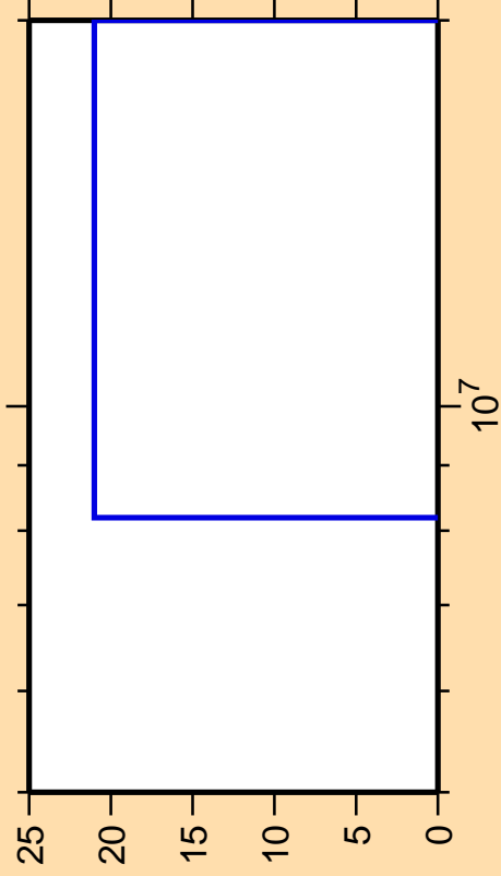
\Delta\sigma/\sigma vs. E for ^{139}\text{La}(n,n_1)
