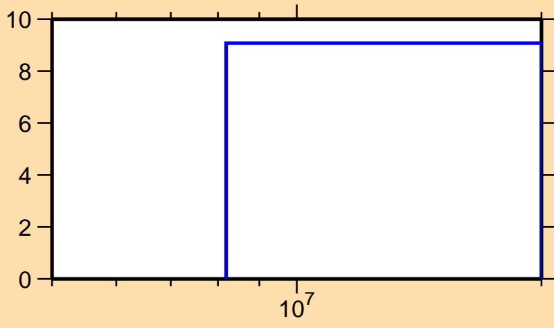
\Delta\sigma/\sigma vs. E for ^{139}\text{La}(n,2n)
