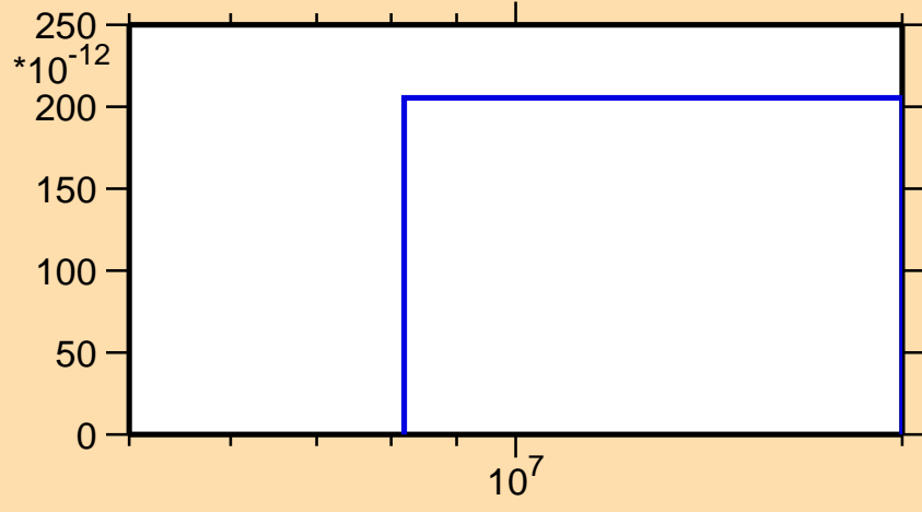
\sigma vs. E for ^{139}\text{La}(n,nt)
