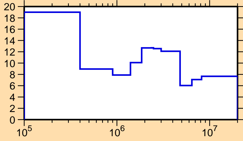
\Delta\sigma/\sigma vs. E for ^{139}\text{La}(n,\text{el.})
