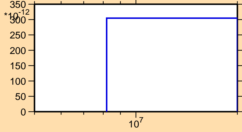
\sigma vs. E for ^{139}\text{La}(n,2np)
