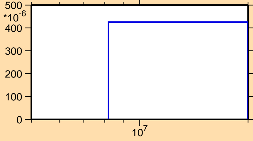
\sigma vs. E for ^{139}\text{La}(n,3n)
