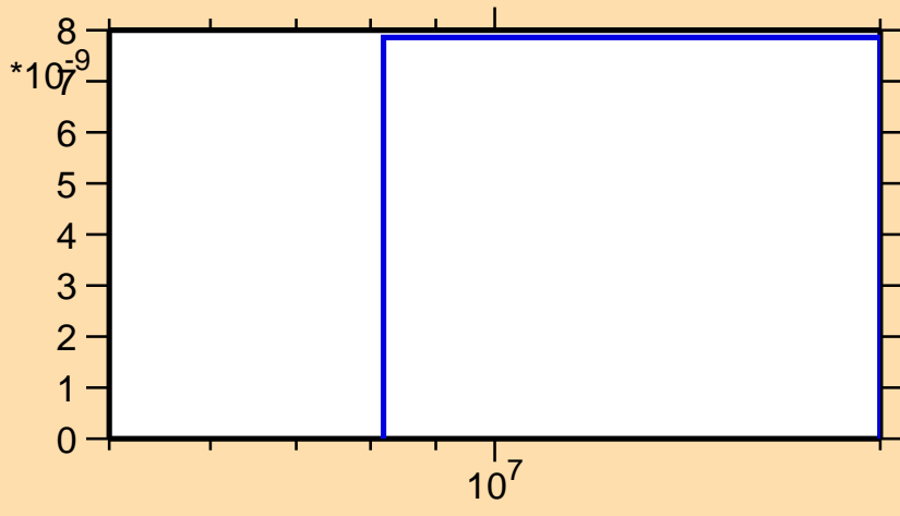
\sigma vs. E for ^{140}\text{La}(n,p\alpha)
