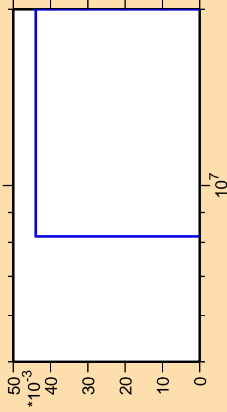
\Delta\sigma/\sigma vs. E for ^{140}\text{La}(\text{mt117})
