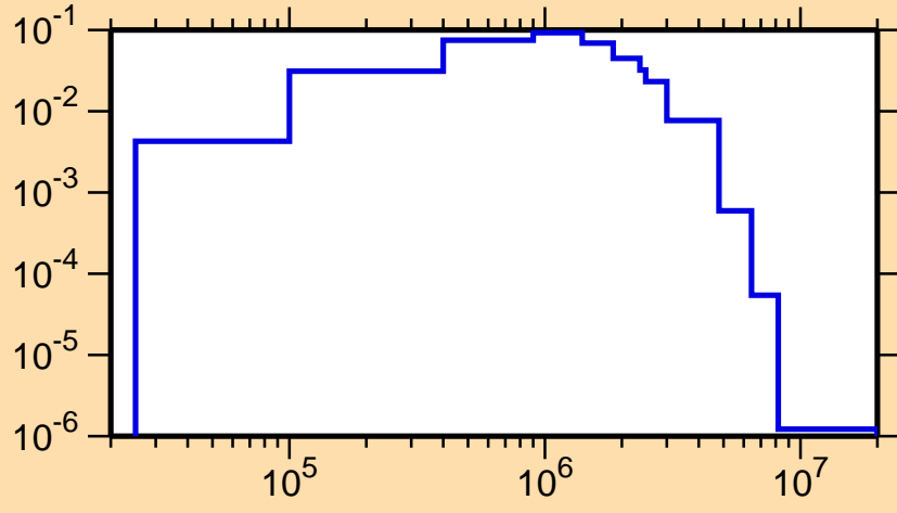
\sigma vs. E for ^{140}\text{La}(n,n_4)
