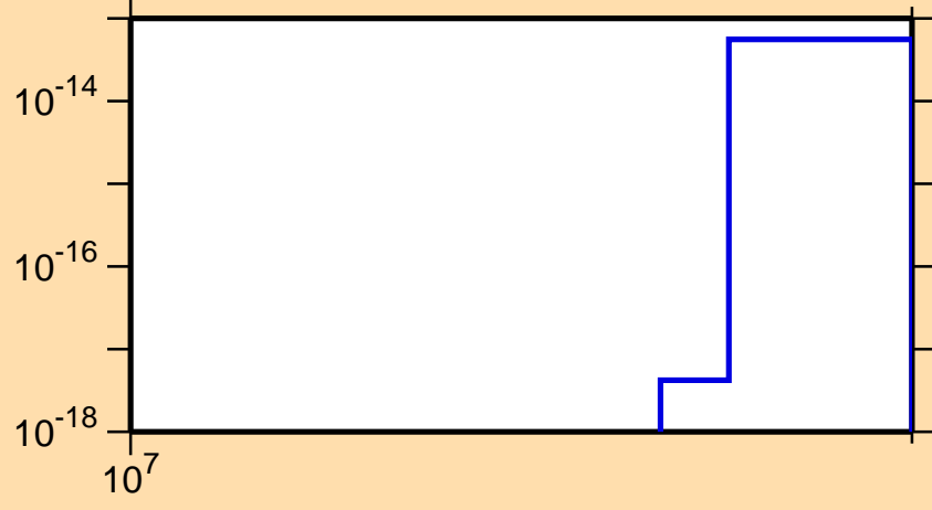
\sigma vs. E for ^{141}\text{La}(n,3n\alpha)
