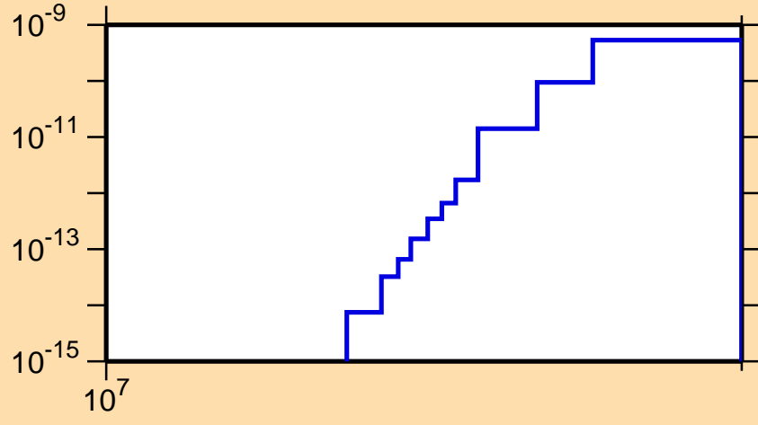
\sigma vs. E for ^{141}\text{La} (mt117)
