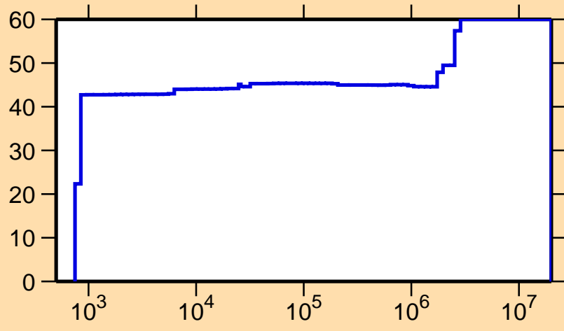
\Delta\sigma/\sigma vs. E for ^{141}\text{La}(n,\gamma)
