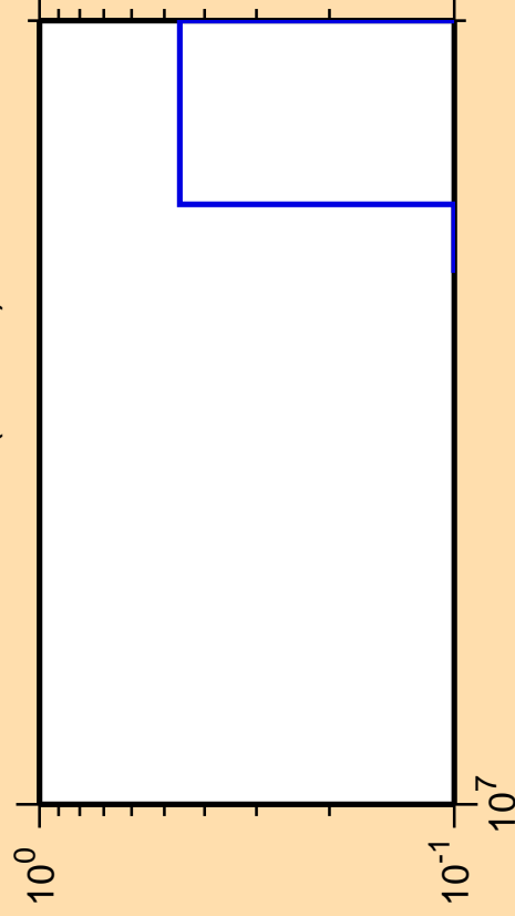
\Delta\sigma/\sigma vs. E for ^{141}\text{La}(n,3n\alpha)
