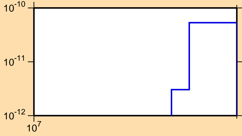
\sigma vs. E for ^{141}\text{La} (mt 45)
