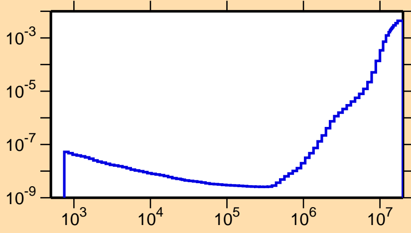
\sigma vs. E for ^{141}\text{La}(n,\alpha)
