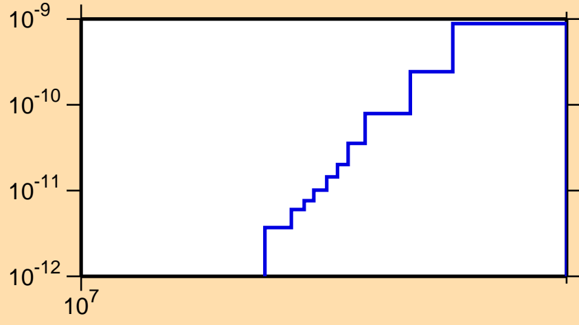
\sigma vs. E for ^{141}\text{La}(n,p\alpha)
