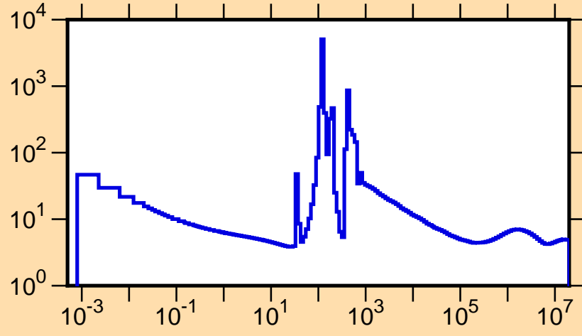
\sigma vs. E for ^{141}\text{La}(n,\text{tot.})
