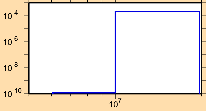
\sigma vs. E for ^{141}\text{La}(n,t)
