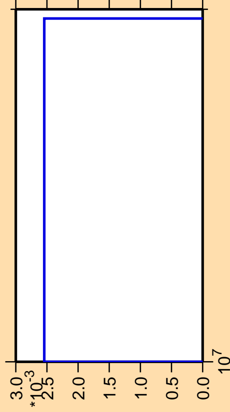
\Delta\sigma/\sigma vs. E for ^{141}\text{La}(n,3n\alpha)
