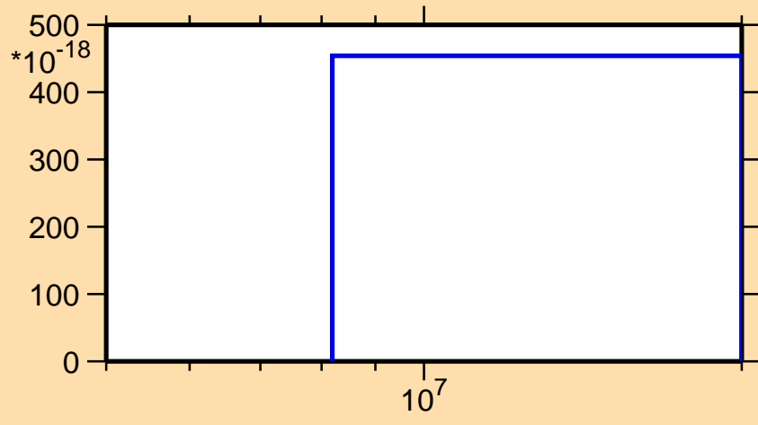
\sigma vs. E for ^{141}\text{La}(n,3n\alpha)
