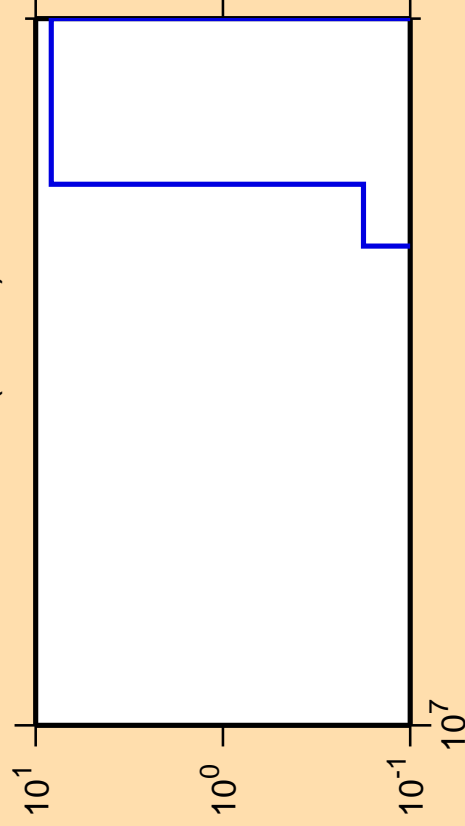
\Delta\sigma/\sigma vs. E for ^{142}\text{La} (mt 45)
