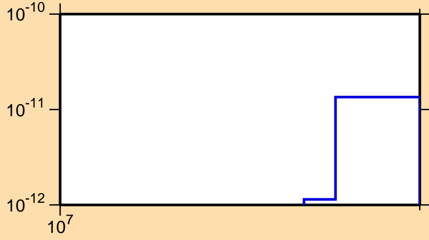
\sigma vs. E for ^{142}\text{La}(\text{mt117})
