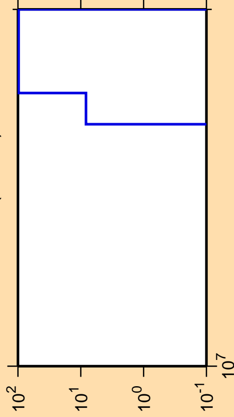
\Delta\sigma/\sigma vs. E for ^{142}\text{La}(\text{mt117})
