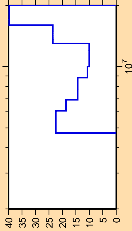
\Delta\sigma/\sigma vs. E for ^{142}\text{La}(n,2n)
