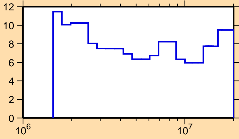
\Delta\sigma/\sigma vs. E for ^{142}\text{La}(n,\text{nonel.})
