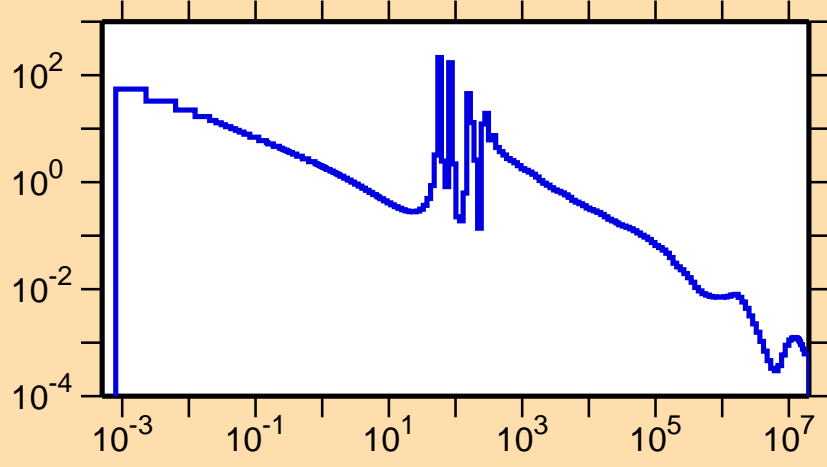
\sigma vs. E for ^{142}\text{La}(n,\gamma)
