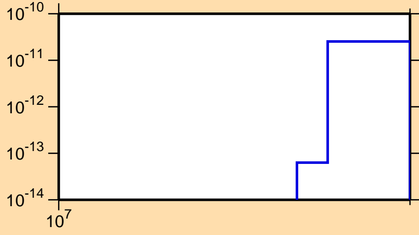
\sigma vs. E for ^{142}\text{La}(n,\text{He3})
