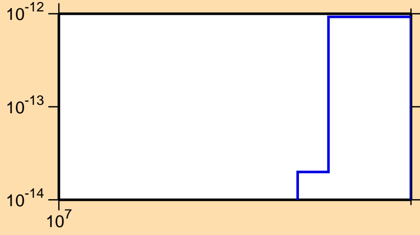
\sigma vs. E for ^{142}\text{La} (mt 45)
