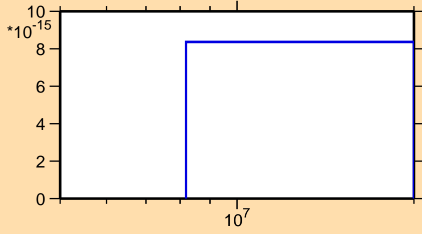
\sigma vs. E for ^{142}\text{La} (mt 45)
