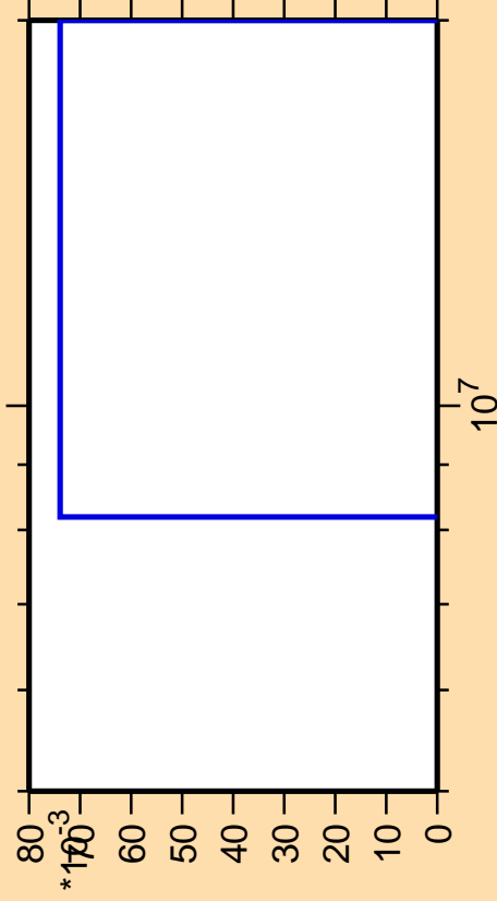
\Delta\sigma/\sigma vs. E for ^{142}\text{La} (mt 45)
