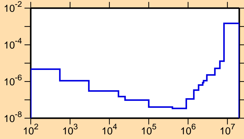
\sigma vs. E for ^{142}\text{La}(n,\alpha)
