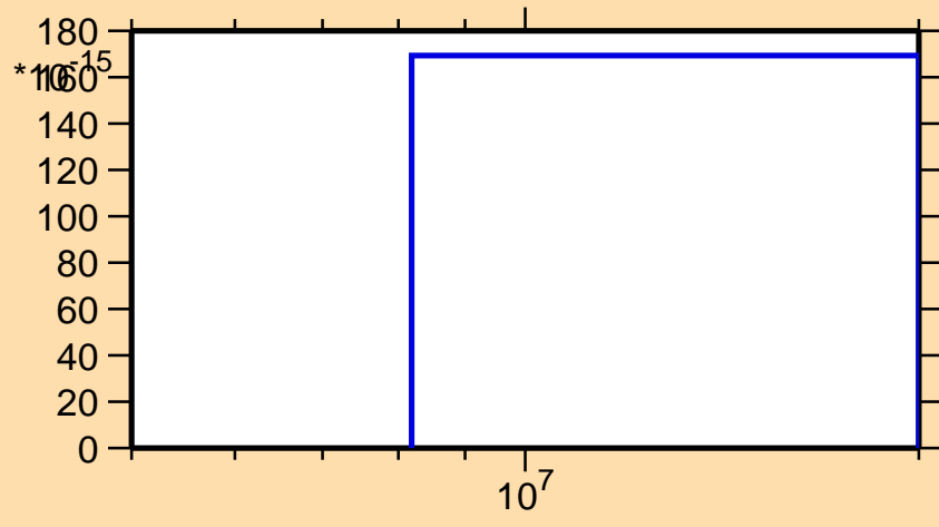
\sigma vs. E for ^{142}\text{La}(\text{mt117})
