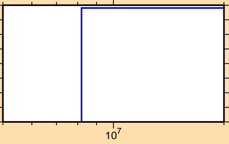
\sigma vs. E for ^{142}\text{La} (mt 11)
