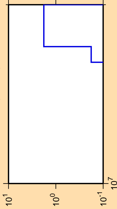
\Delta\sigma/\sigma vs. E for ^{143}\text{La}(\text{mt117})
