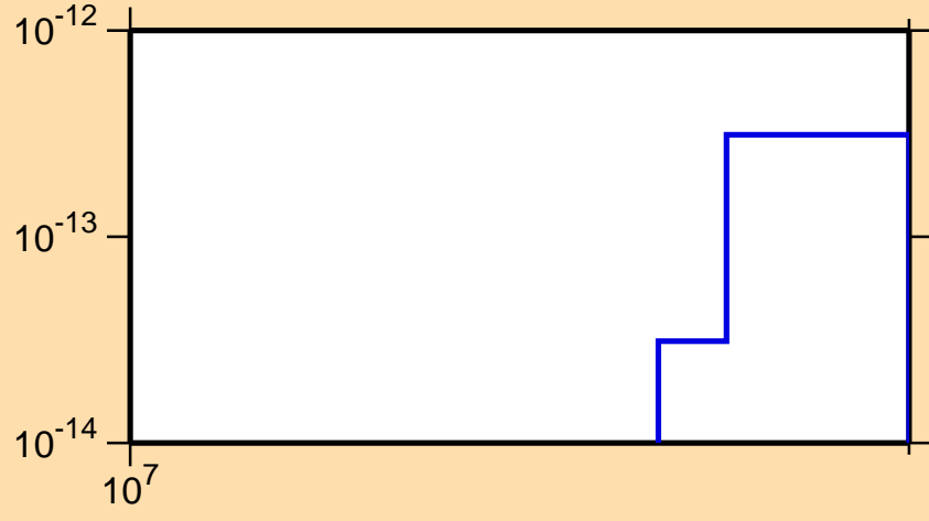
\sigma vs. E for ^{143}\text{La}(\text{mt117})
