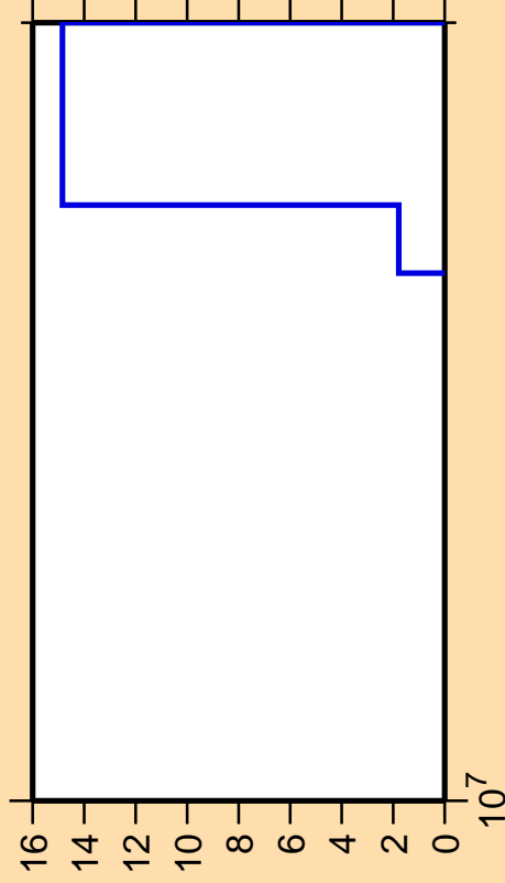
\Delta\sigma/\sigma vs. E for ^{143}\text{La}(n,p\alpha)
