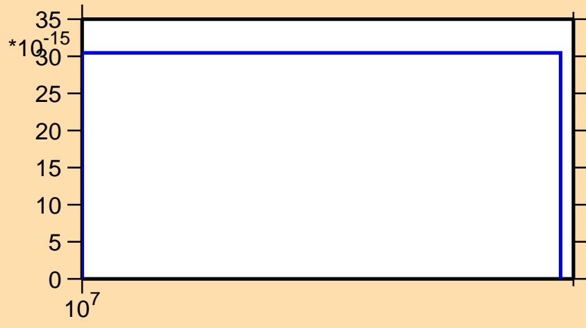
\sigma vs. E for ^{143}\text{La}(n,p\alpha)
