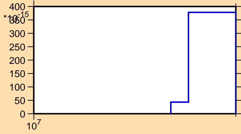
\sigma vs. E for ^{144}\text{La}(n,p\alpha)
