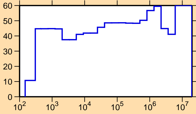
\Delta\sigma/\sigma vs. E for ^{144}\text{La}(n,\gamma)
