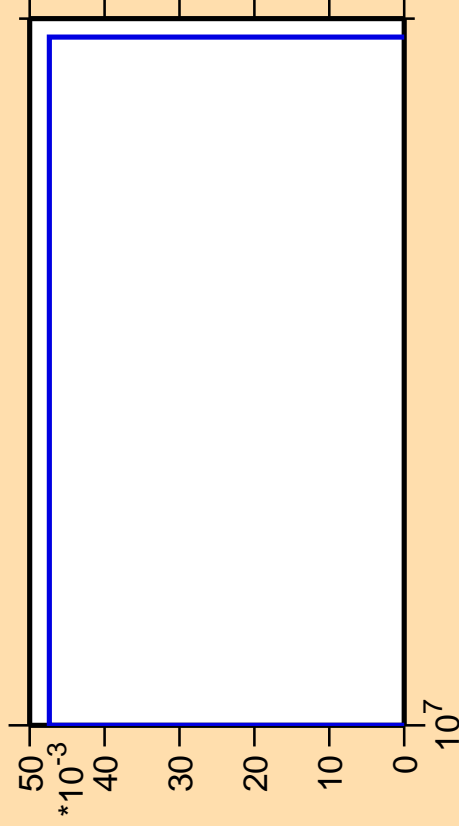
\Delta\sigma/\sigma vs. E for ^{144}\text{La}(n,p\alpha)
