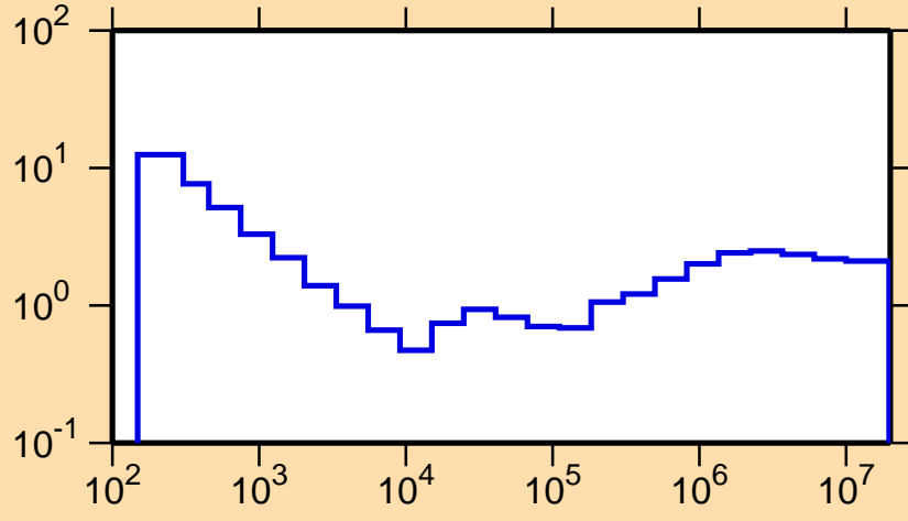
\sigma vs. E for ^{144}\text{La}(n,\text{nonel.})
