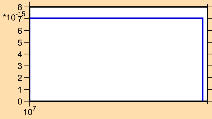
\sigma vs. E for ^{144}\text{La}(n,p\alpha)
