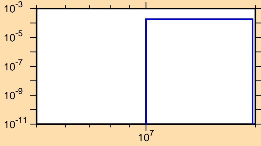
\sigma vs. E for ^{144}\text{La}(n,np)
