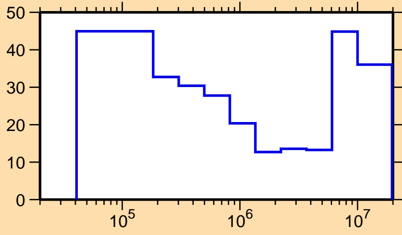
\Delta\sigma/\sigma vs. E for ^{145}\text{La}(n,\text{inel.})
