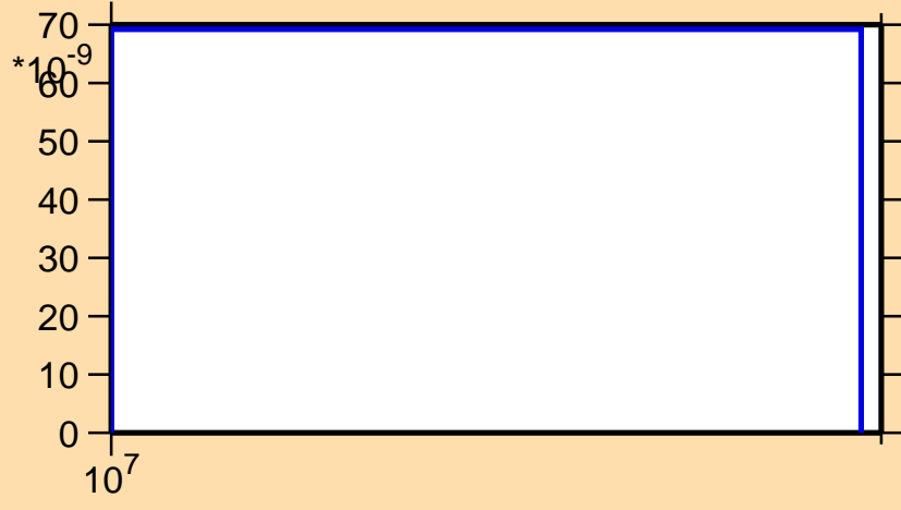
\sigma vs. E for ^{145}\text{La}(n,\text{nd})
