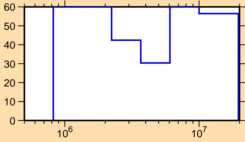
\Delta\sigma/\sigma vs. E for ^{145}\text{La}(n,n\text{cont.})
