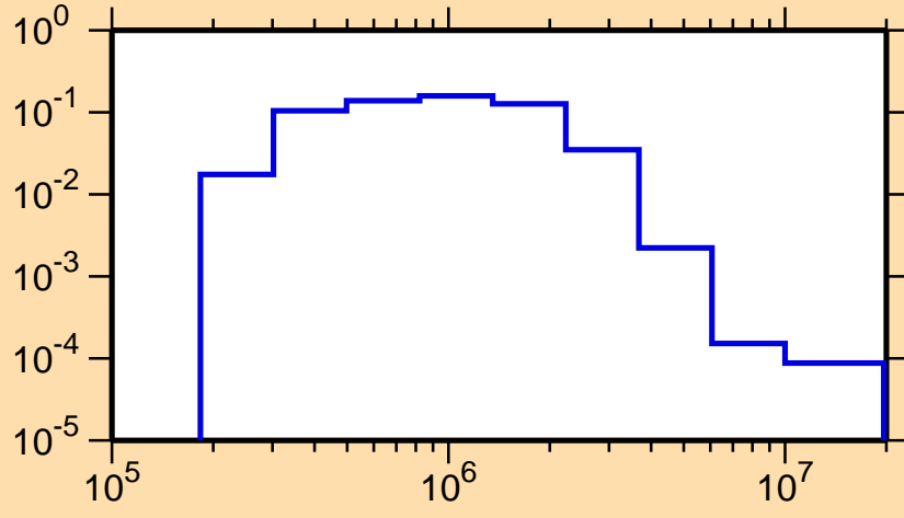
\sigma vs. E for ^{145}\text{La}(n,n_4)
