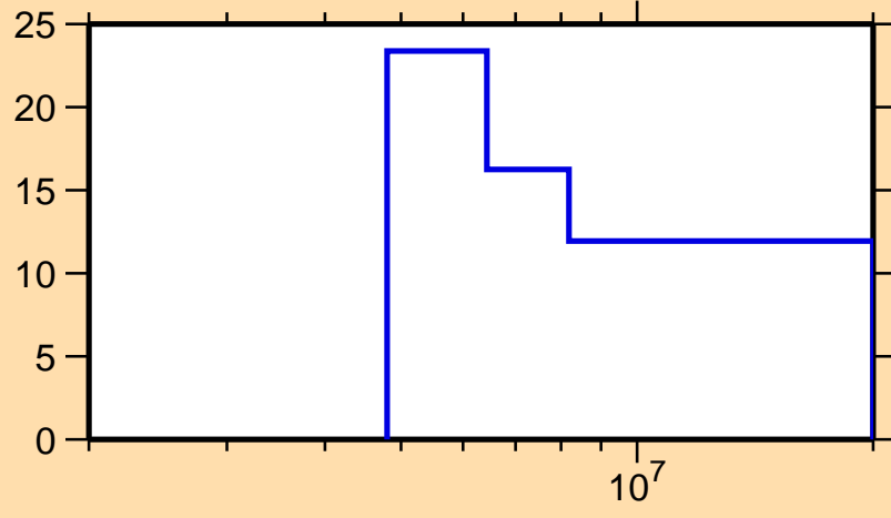
\Delta\sigma/\sigma vs. E for ^{145}\text{La}(n,\text{tot.})
