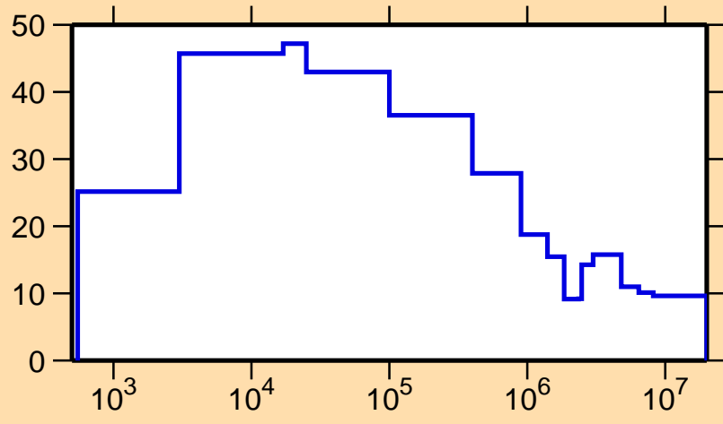
\Delta\sigma/\sigma vs. E for ^{145}\text{La}(n,\text{nonel.})
