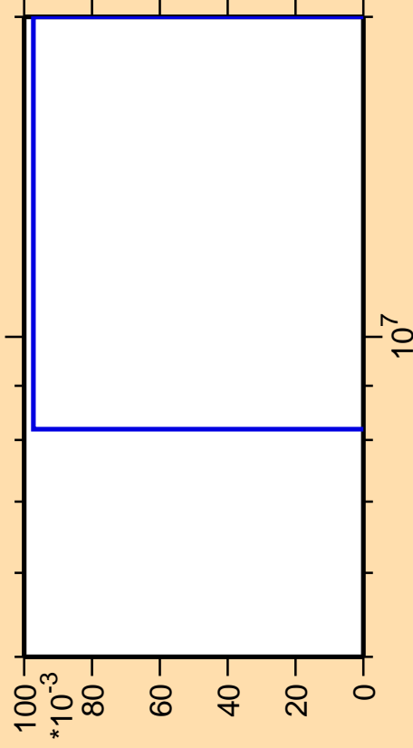
\Delta\sigma/\sigma vs. E for ^{145}\text{La} (mt 11)
