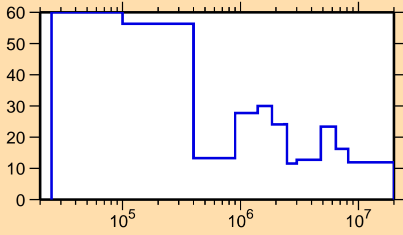
\Delta\sigma/\sigma vs. E for ^{145}\text{La}(n,\text{tot.})
