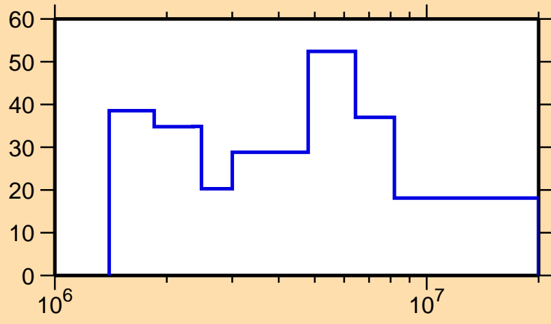
\Delta\sigma/\sigma vs. E for ^{145}\text{La}(n,\text{el.})
