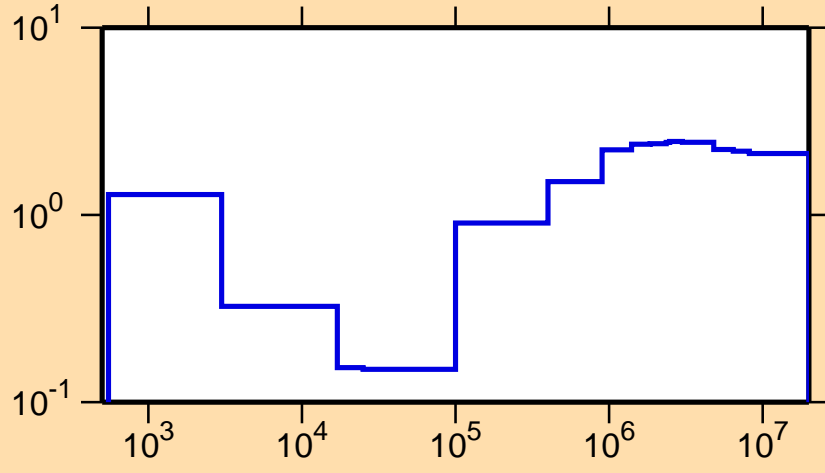
\sigma vs. E for ^{145}\text{La}(n,\text{nonel.})
