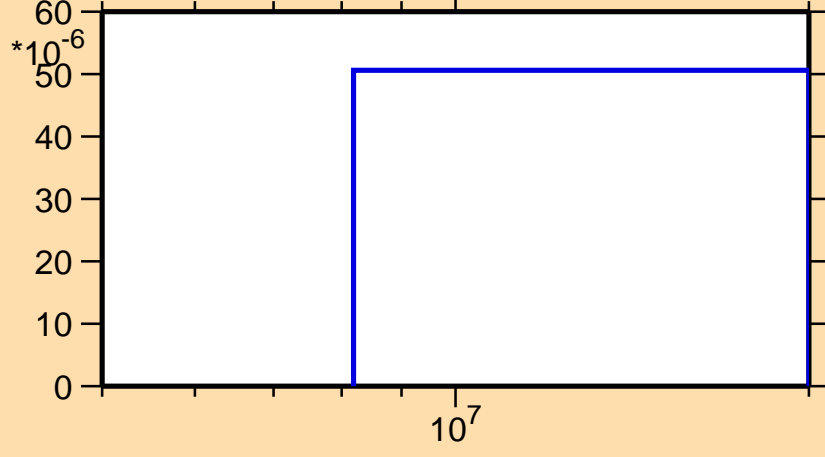
\sigma vs. E for ^{145}\text{La}(n,t)
