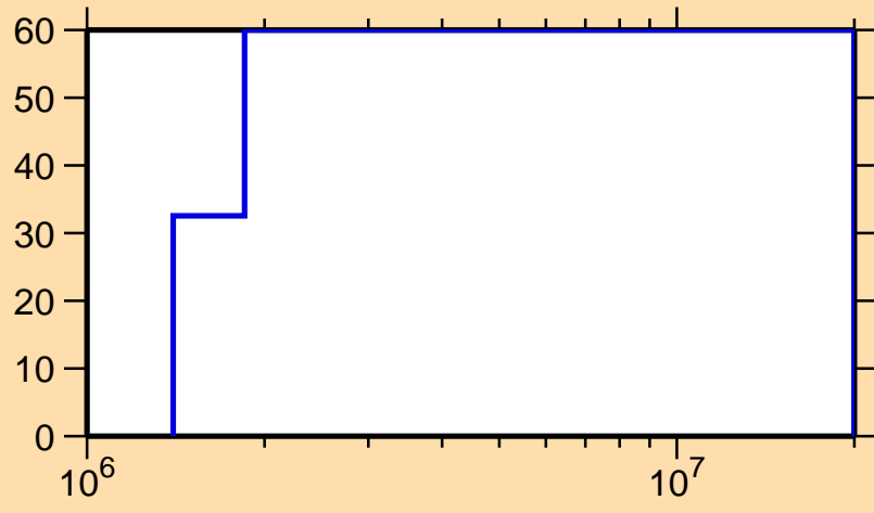
\Delta\sigma/\sigma vs. E for ^{145}\text{La}(n,n_1)
