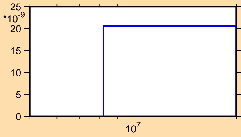
\sigma vs. E for ^{145}\text{La}(n,2n\alpha)
