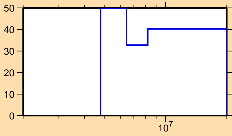
\Delta\sigma/\sigma vs. E for ^{145}\text{La}(n,2n)
