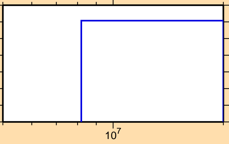
\sigma vs. E for ^{145}\text{La}(n,\text{nd})
