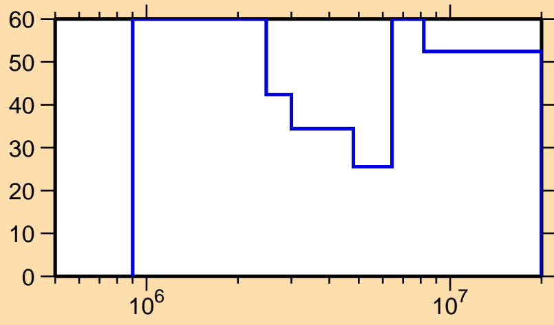
\Delta\sigma/\sigma vs. E for ^{145}\text{La}(n,n\text{cont.})
