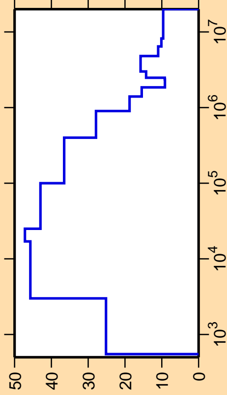
\Delta\sigma/\sigma vs. E for ^{145}\text{La}(n,\text{nonel.})
