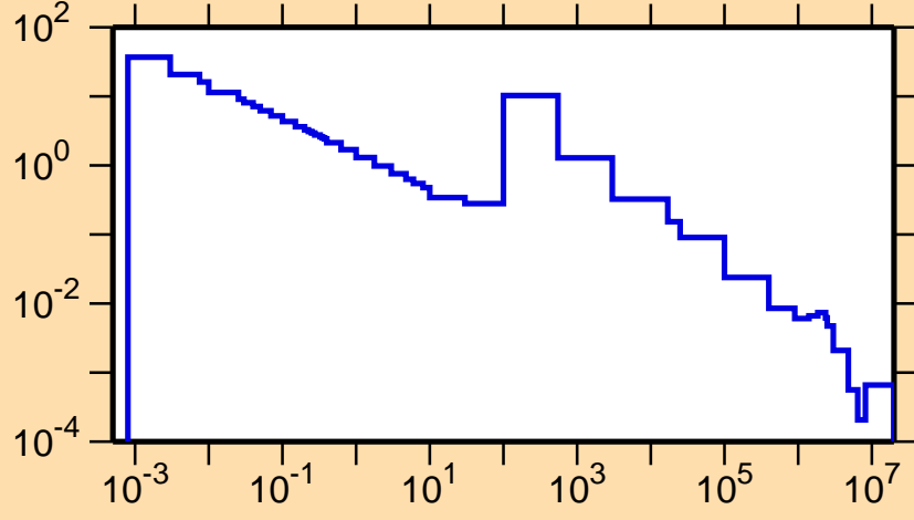
\sigma vs. E for ^{145}\text{La}(n,\gamma)
