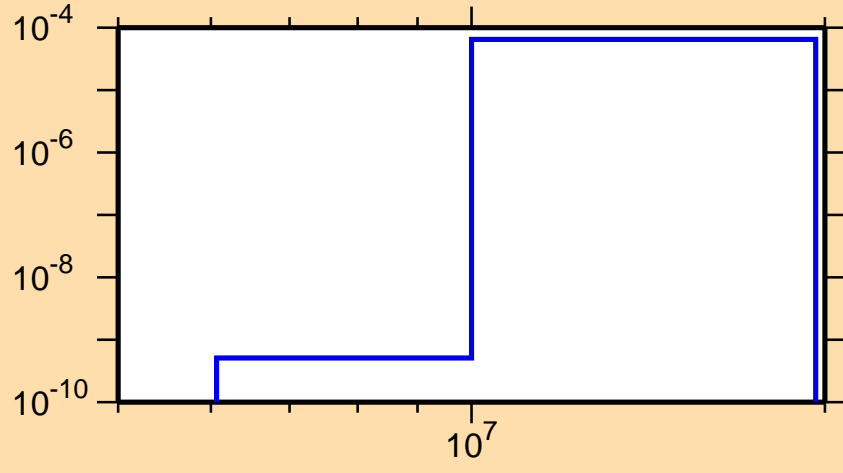
\sigma vs. E for ^{146}\text{La}(n,n\alpha)
