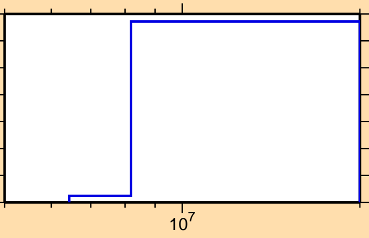
\sigma vs. E for ^{146}\text{La}(n,n\alpha)
