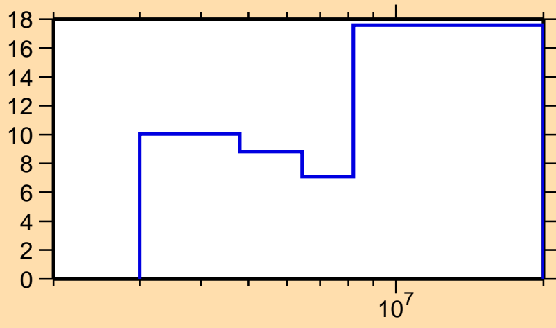
\Delta\sigma/\sigma vs. E for ^{146}\text{La}(n,2n)
