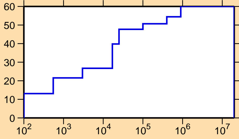
\Delta\sigma/\sigma vs. E for ^{146}\text{La}(n,\gamma)
