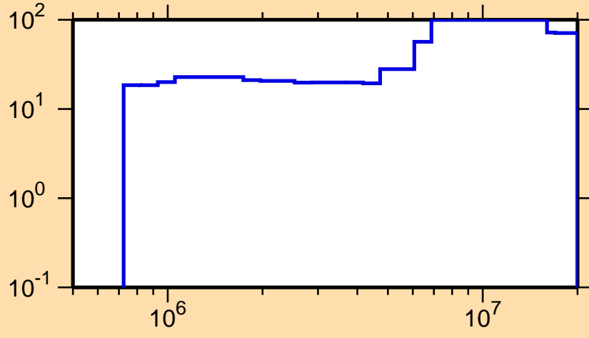
\Delta\sigma/\sigma vs. E for ^{147}\text{La}(n,\text{inel.})
