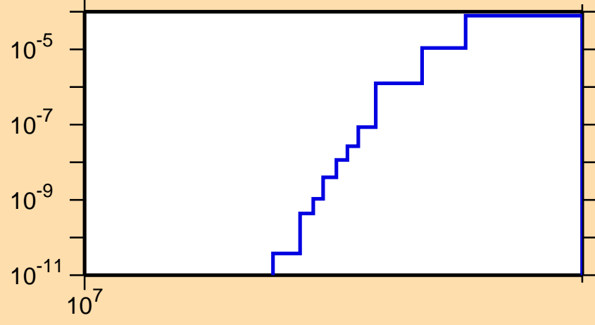
\sigma vs. E for ^{147}\text{La}(n,nt)
