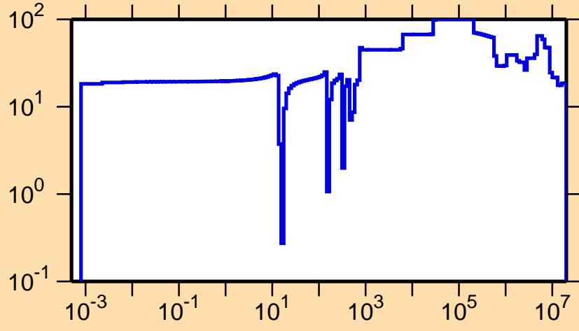
\Delta\sigma/\sigma vs. E for ^{147}\text{La}(n,\text{el.})
