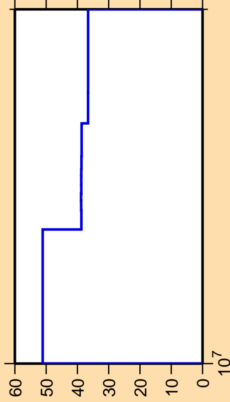
\Delta\sigma/\sigma vs. E for ^{147}\text{La}(n,3n)
