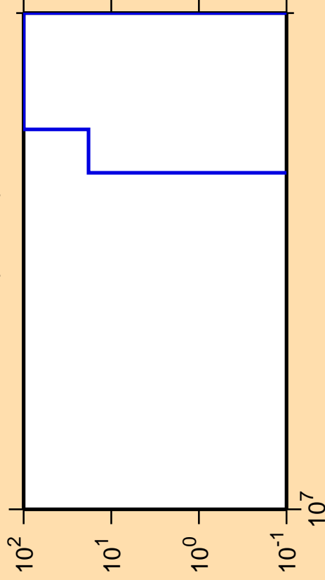
\Delta\sigma/\sigma vs. E for ^{147}\text{La}(n,3n\alpha)
