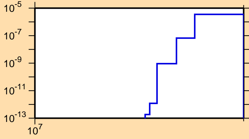
\sigma vs. E for ^{147}\text{La}(n,\text{nd})
