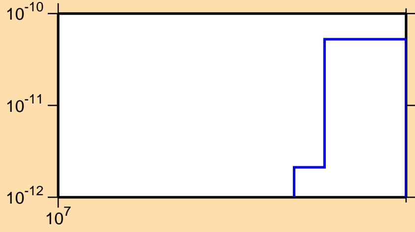
\sigma vs. E for ^{147}\text{La}(n,3n\alpha)
