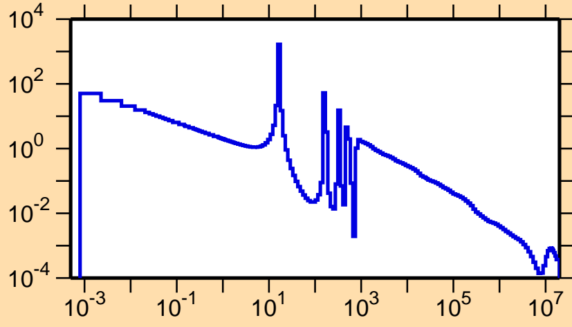
\sigma vs. E for ^{147}\text{La}(n,\gamma)
