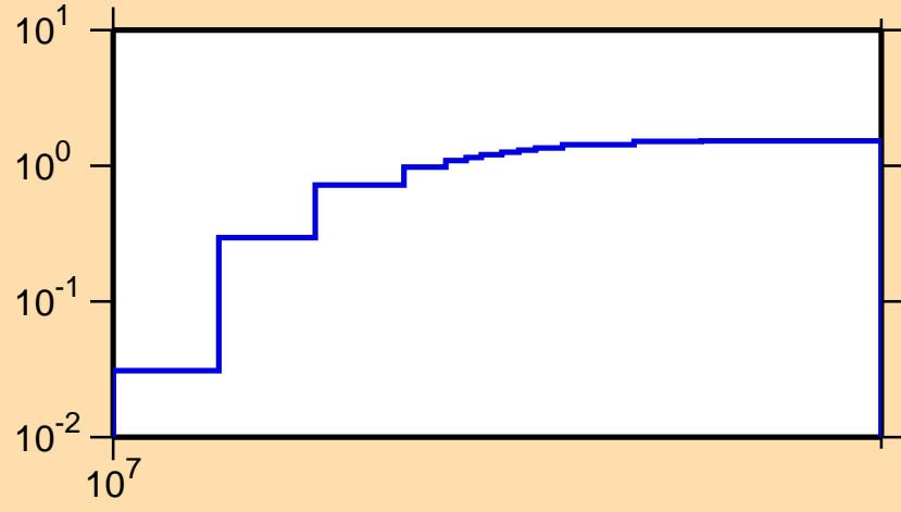
\sigma vs. E for ^{147}\text{La}(n,3n)
