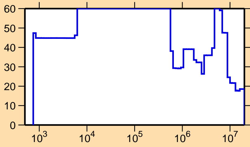
\Delta\sigma/\sigma vs. E for ^{147}\text{La}(n,\text{el.})
