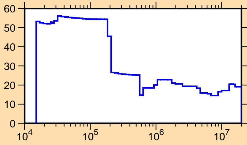
\Delta\sigma/\sigma vs. E for ^{147}\text{La}(n,\text{nonel.})
