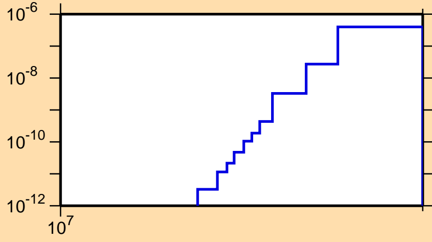
\sigma vs. E for ^{147}\text{La}(n,2n\alpha)
