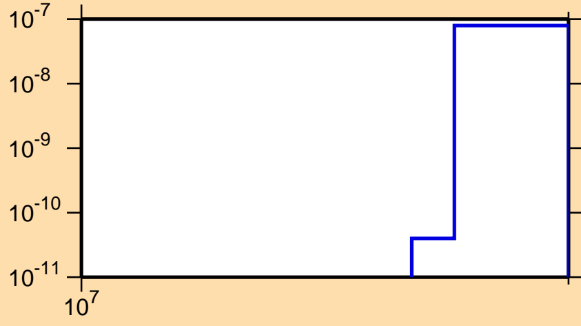
\sigma vs. E for ^{147}\text{La}(n,2np)
