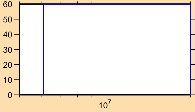
\Delta\sigma/\sigma vs. E for ^{147}\text{La}(n,\gamma)
