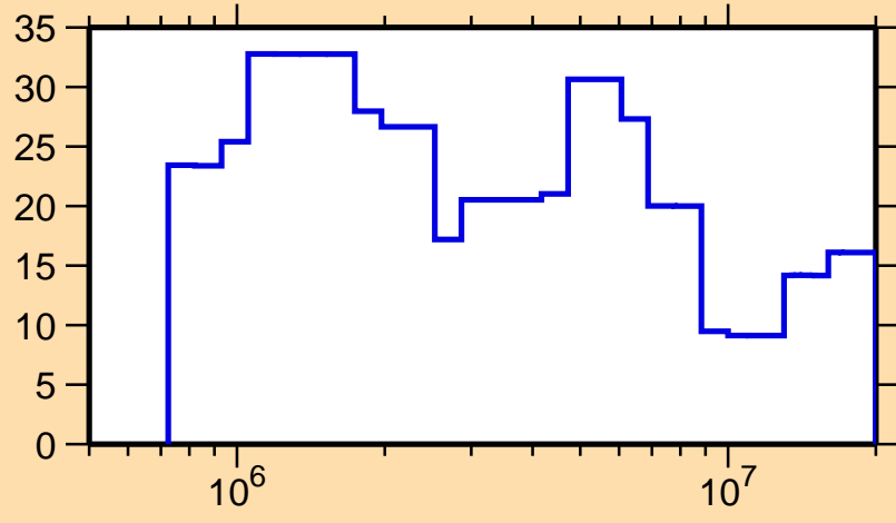
\Delta\sigma/\sigma vs. E for ^{147}\text{La}(n,\text{tot.})
