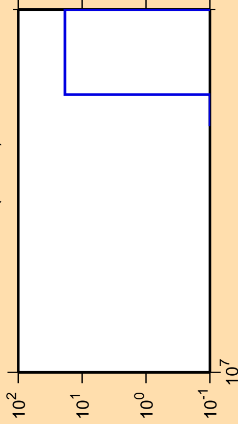
\Delta\sigma/\sigma vs. E for ^{147}\text{La} (mt 11)
