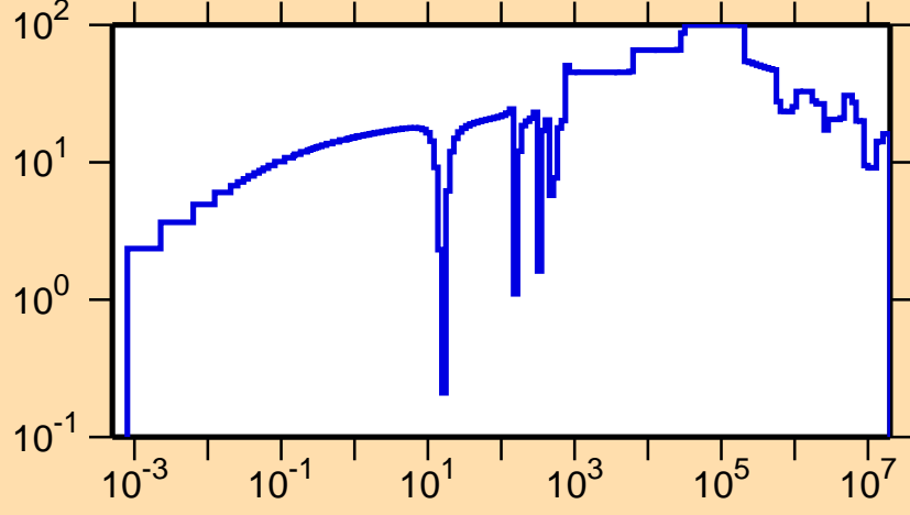
\Delta\sigma/\sigma vs. E for ^{147}\text{La}(n,\text{tot.})
