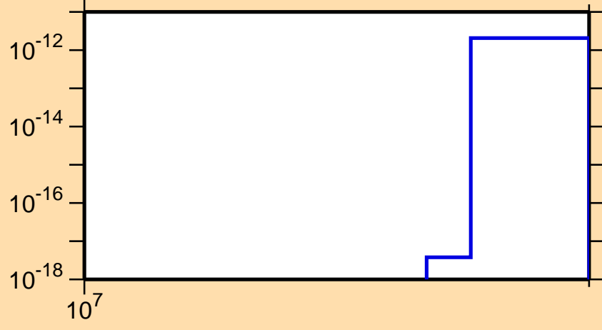
\sigma vs. E for ^{147}\text{La} (mt 11)
