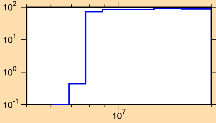
\Delta\sigma/\sigma vs. E for ^{147}\text{La}(n,p)
