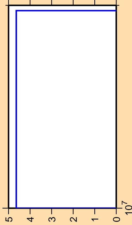
\Delta\sigma/\sigma vs. E for ^{147}\text{La}(n,3n\alpha)
