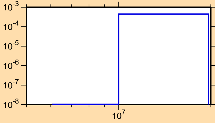
\sigma vs. E for ^{147}\text{La}(n,p)
