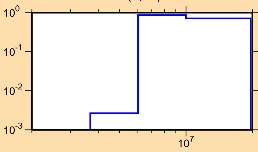
\sigma vs. E for ^{147}\text{La}(n,2n)
