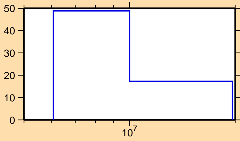
\Delta\sigma/\sigma vs. E for ^{147}\text{La}(n,el.)
