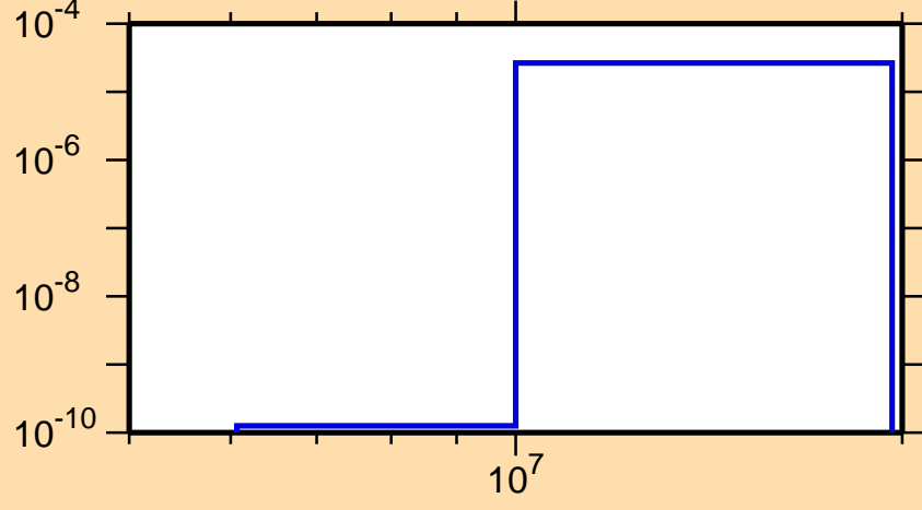
\sigma vs. E for ^{147}\text{La}(n,n\alpha)
