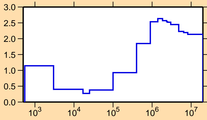
\sigma vs. E for ^{147}\text{La}(n,\text{nonel.})
