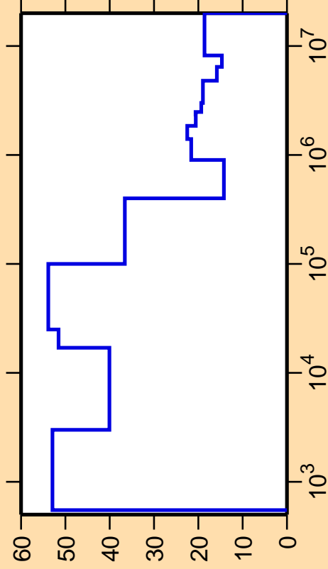
\Delta\sigma/\sigma vs. E for ^{147}\text{La}(n,\text{nonel.})
