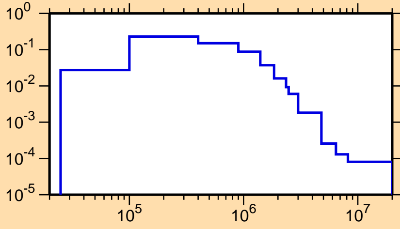
\sigma vs. E for ^{147}\text{La}(n,n_2)
