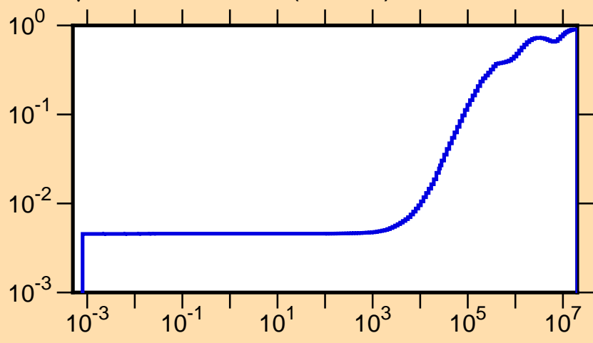
\mu vs. E for ^{148}\text{La}(\text{mt251})
