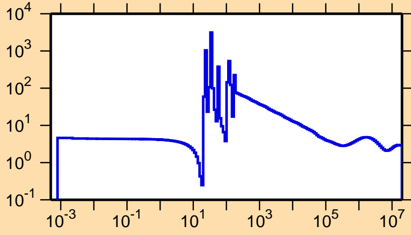
\sigma vs. E for ^{148}\text{La}(n,\text{el.})
