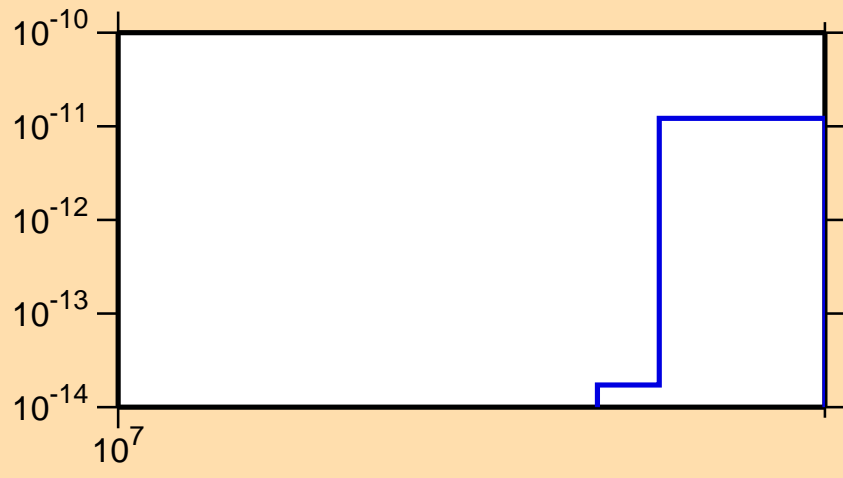
\sigma vs. E for ^{148}\text{La}(n,3n\alpha)
