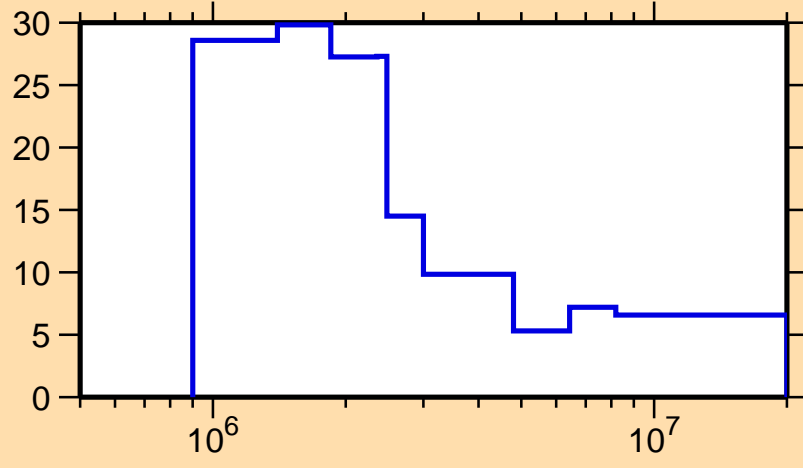
\Delta\sigma/\sigma vs. E for ^{148}\text{La}(n,\text{nonel.})
