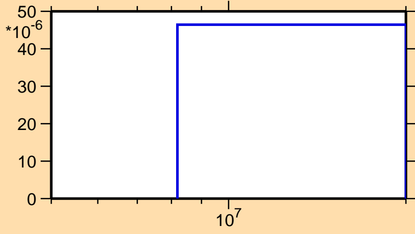
\sigma vs. E for ^{148}\text{La}(n,d)
