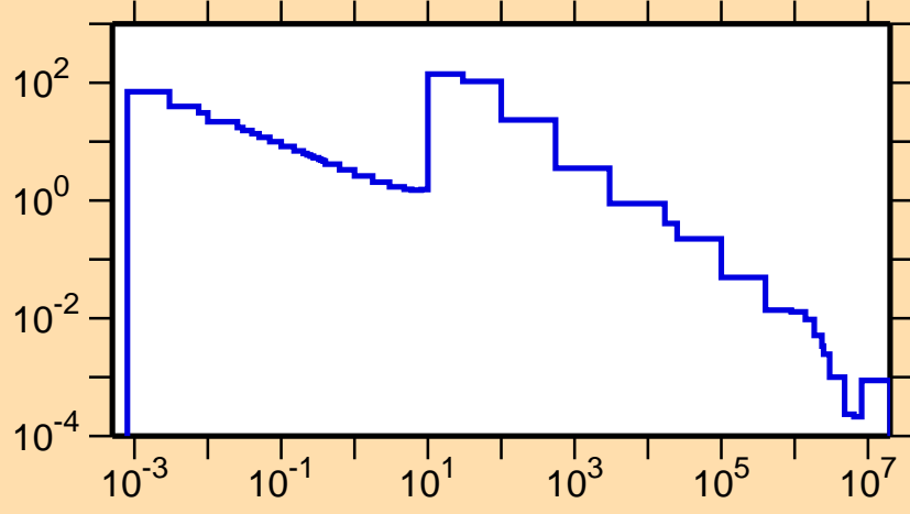
\sigma vs. E for ^{148}\text{La}(n,\gamma)
