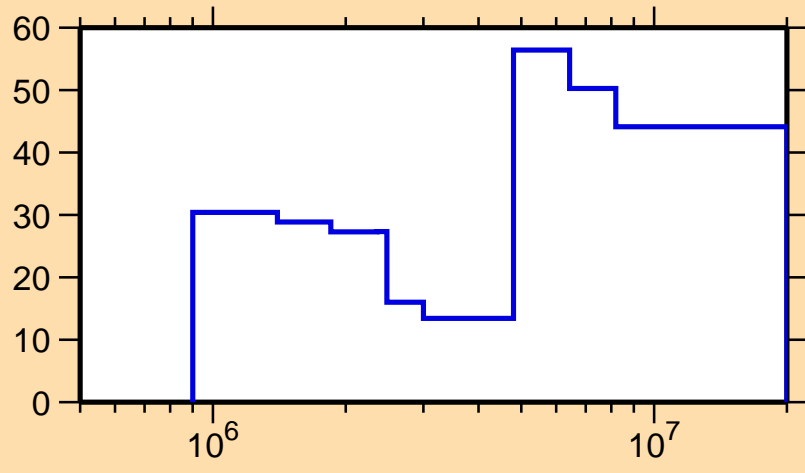
\Delta\sigma/\sigma vs. E for ^{148}\text{La}(n,\text{inel.})
