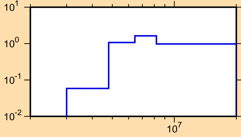
\sigma vs. E for ^{148}\text{La}(n,2n)
