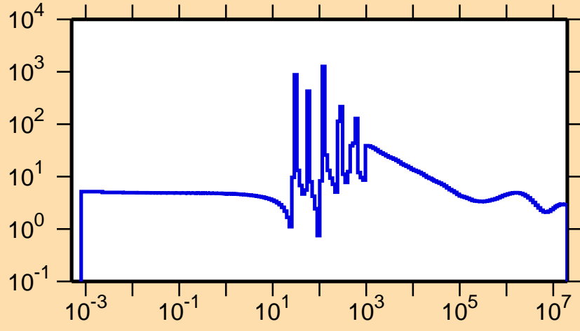
\sigma vs. E for ^{149}\text{La}(n,\text{el.})
