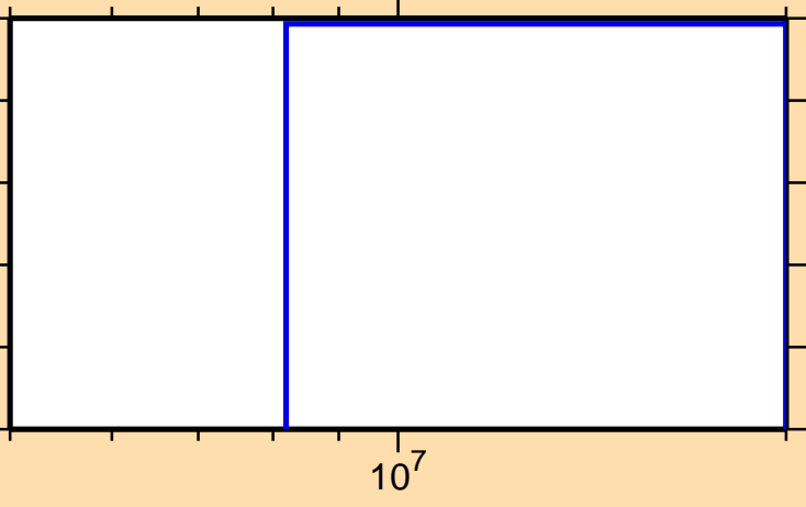
\sigma vs. E for ^{149}\text{La}(n,\text{nd})
