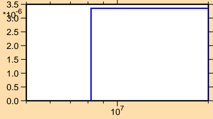
\sigma vs. E for ^{149}\text{La}(n,n\alpha)
