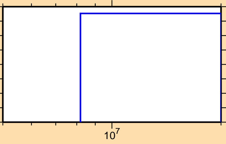
\sigma vs. E for ^{149}\text{La}(n,2np)
