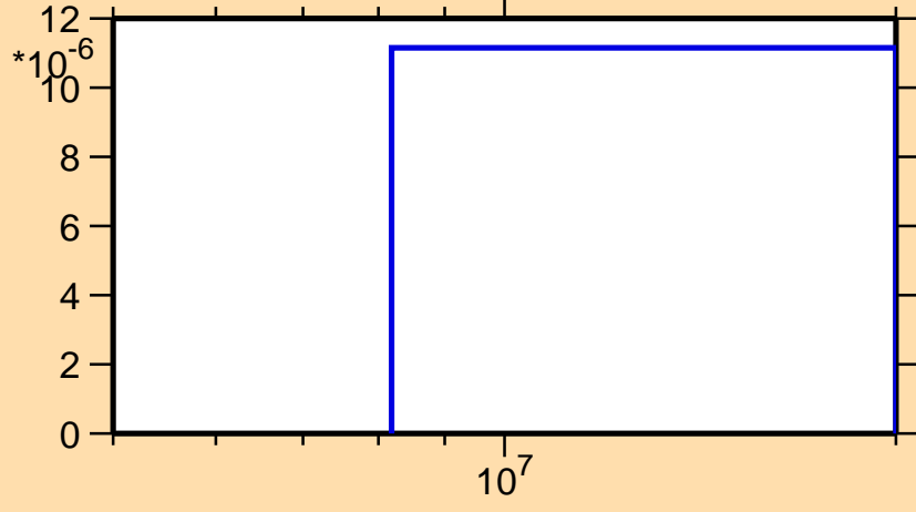
\sigma vs. E for ^{149}\text{La}(n,t)
