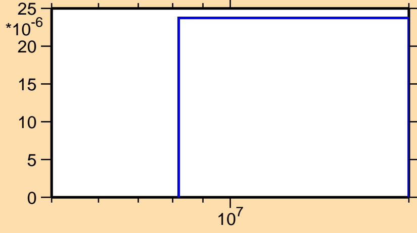
\sigma vs. E for ^{149}\text{La}(n,d)
