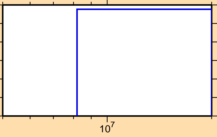
\sigma vs. E for ^{149}\text{La}(n,nt)
