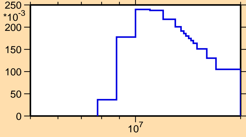
\sigma vs. E for ^{253}\text{Lw}(n,2n)
