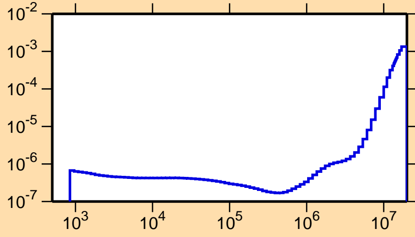
\sigma vs. E for ^{253}\text{Lw}(n,p\alpha)
