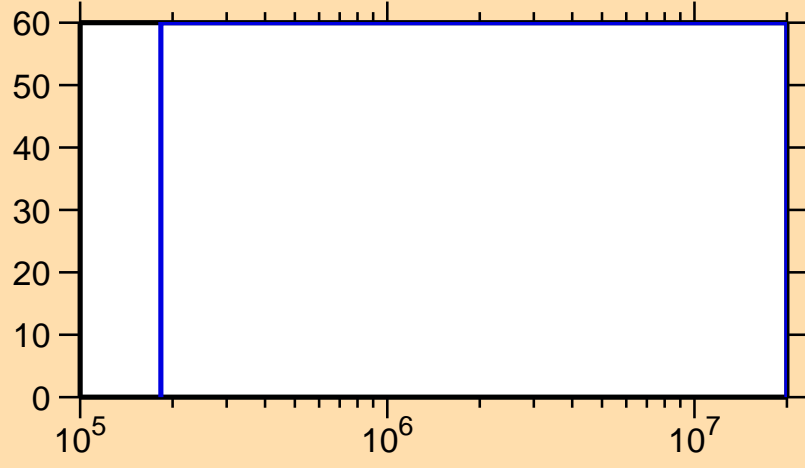
\Delta\sigma/\sigma vs. E for ^{253}\text{Lw}(n,n\text{cont.})
