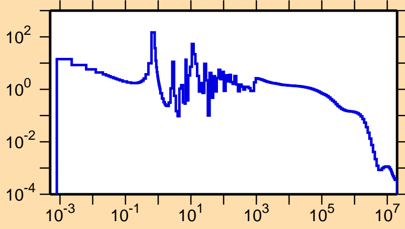
\sigma vs. E for ^{253}\text{Lw}(n,\gamma)
