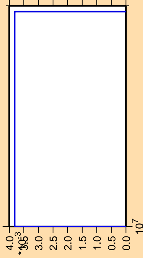
\Delta\sigma/\sigma vs. E for ^{253}\text{Lw} (mt 42)
