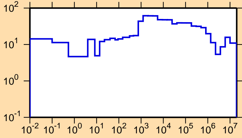
\Delta\sigma/\sigma vs. E for ^{253}\text{Lw}(n,tot.)
