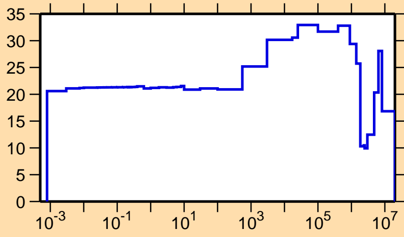
\Delta\sigma/\sigma vs. E for ^{253}\text{Lw}(n,el.)
