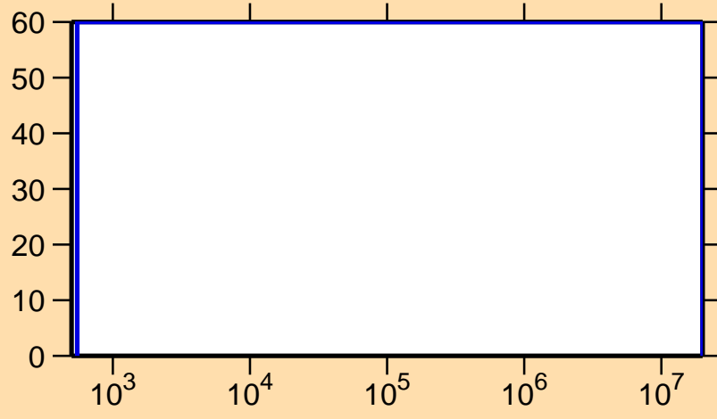
\Delta\sigma/\sigma vs. E for ^{253}\text{Lw}(n,p)
