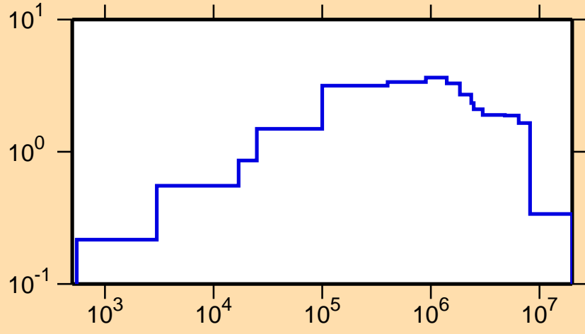
\sigma vs. E for ^{253}\text{Lw}(n,\text{inel.})
