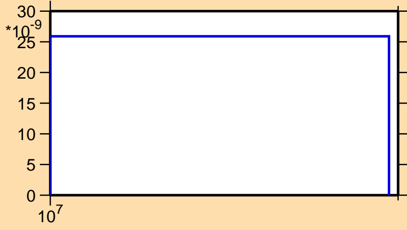
\sigma vs. E for ^{254}\text{Lw}(n,nt)
