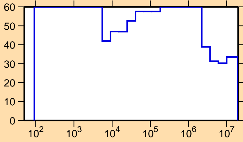
\Delta\sigma/\sigma vs. E for ^{254}\text{Lw}(n,p)
