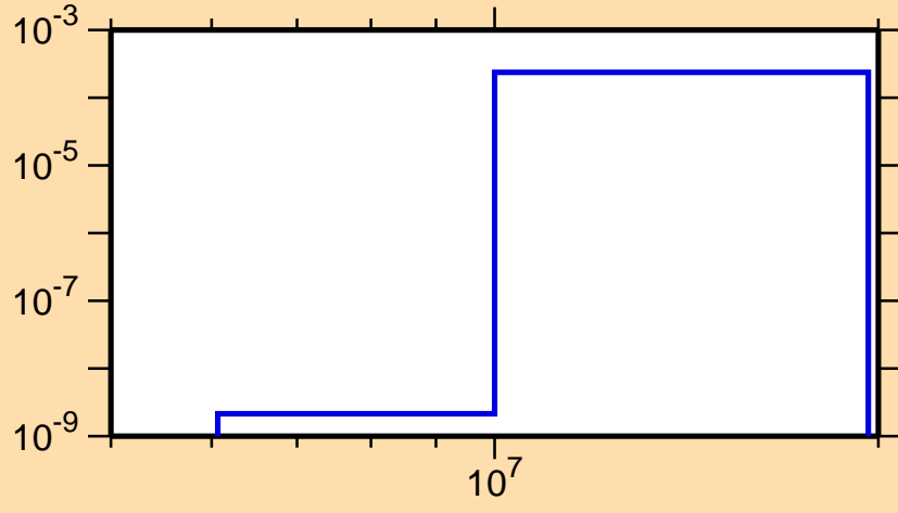
\sigma vs. E for ^{254}\text{Lw}(n,t)
