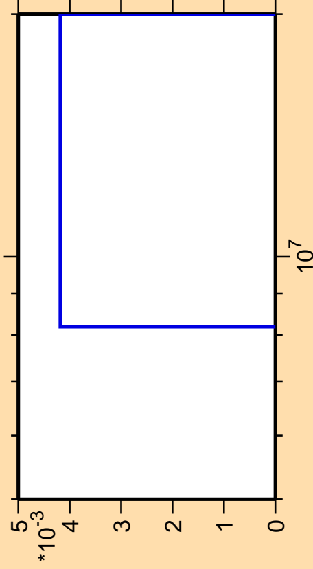
\Delta\sigma/\sigma vs. E for ^{254}\text{Lw}(\text{mt } 11)
