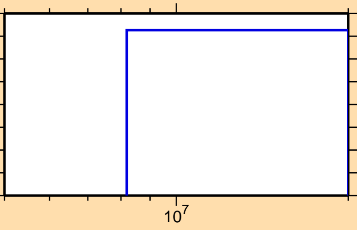
\sigma vs. E for ^{254}\text{Lw}(n,pd)
