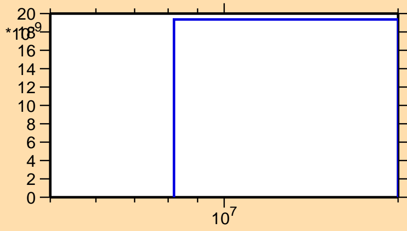
\sigma vs. E for ^{254}\text{Lw}(n,\text{He3})
