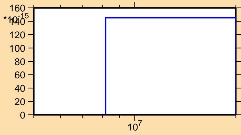
\sigma vs. E for ^{254}\text{Lw}(n,pd)
