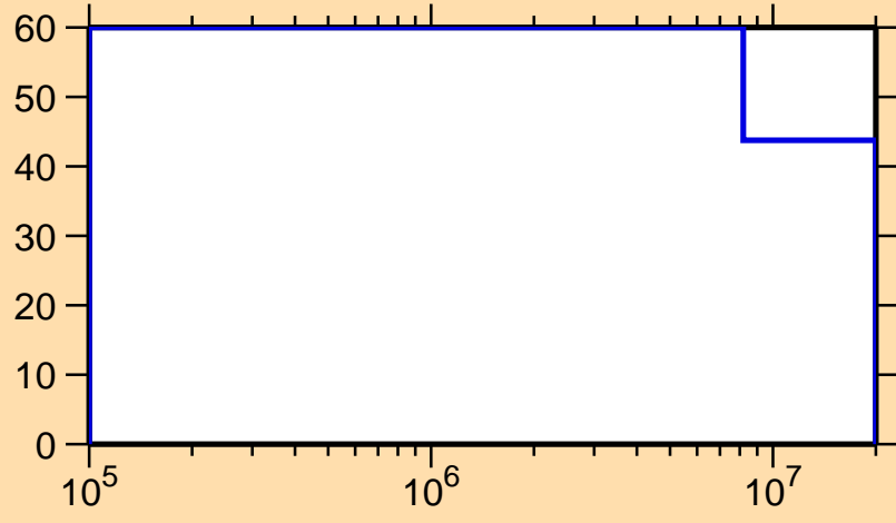
\Delta\sigma/\sigma vs. E for ^{254}\text{Lw}(n,f)
