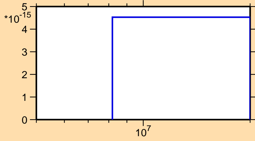
\sigma vs. E for ^{254}\text{Lw}(\text{mt } 11)
