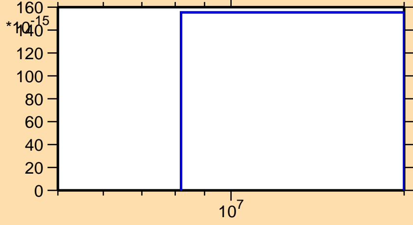
\sigma vs. E for ^{254}\text{Lw}(n,pt)
