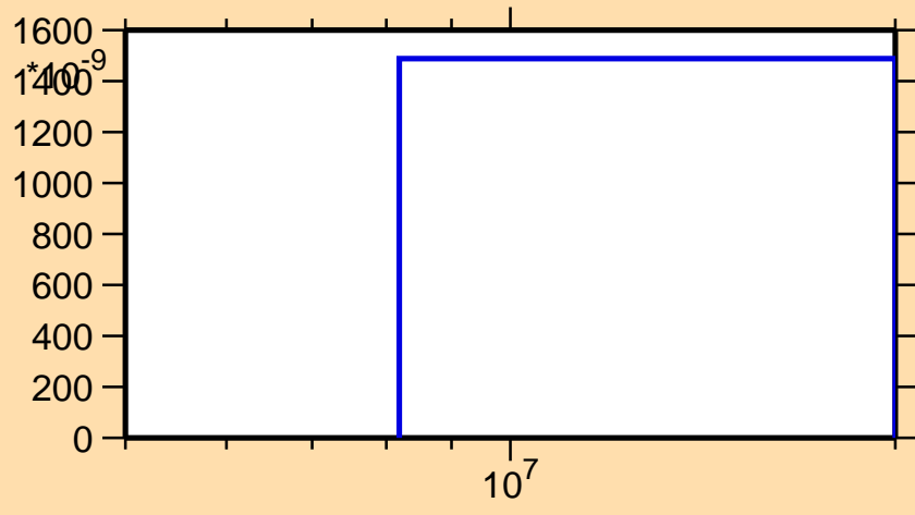
\sigma vs. E for ^{254}\text{Lw}(n,nd)
