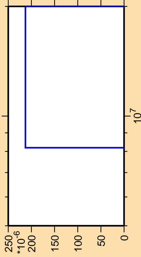
\Delta\sigma/\sigma vs. E for ^{254}\text{Lw}(\text{mt } 42)
