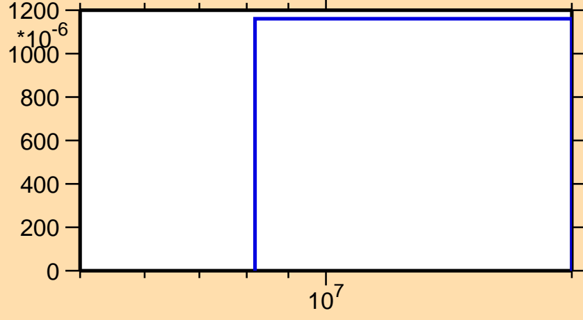
\sigma vs. E for ^{254}\text{Lw}(n,3n)
