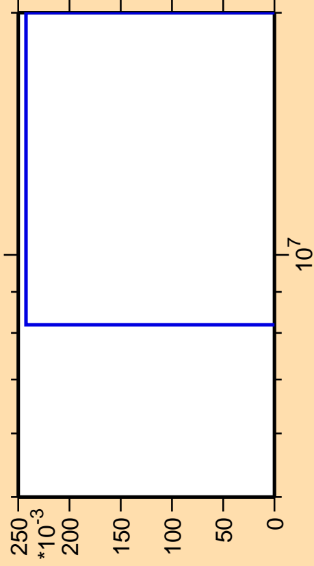
\Delta\sigma/\sigma vs. E for ^{254}\text{Lw}(n,pd)
