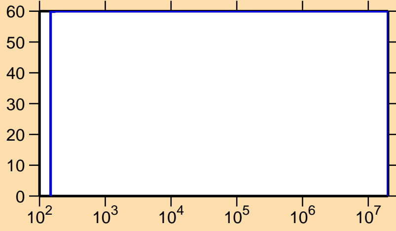
\Delta\sigma/\sigma vs. E for ^{255}\text{Lw}(n,p)
