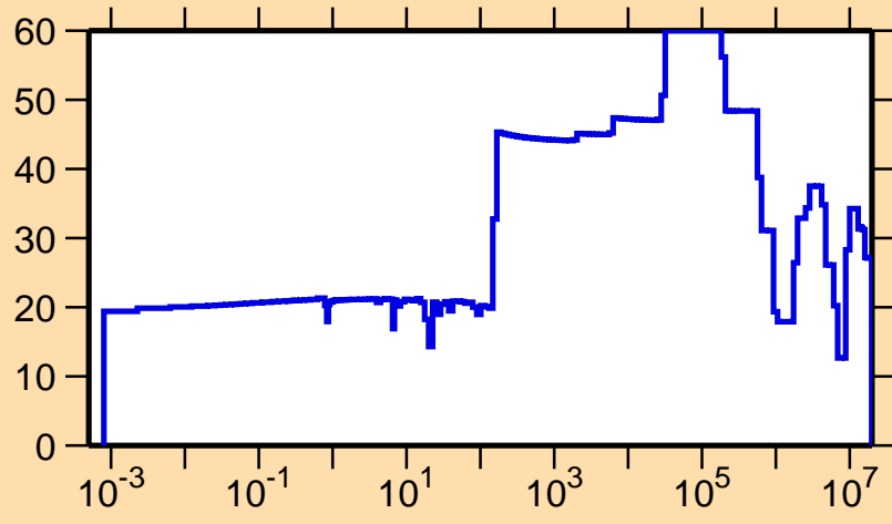
\Delta\sigma/\sigma vs. E for ^{255}\text{Lw}(n,el.)
