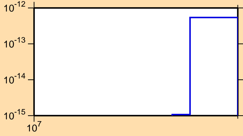
\sigma vs. E for ^{255}\text{Lw}(\text{mt } 11)
