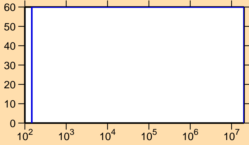
\Delta\sigma/\sigma vs. E for ^{255}\text{Lw}(n,\gamma)
