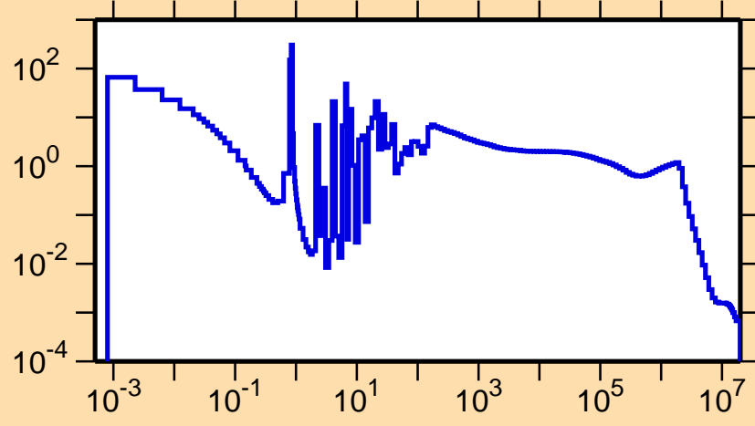
\sigma vs. E for ^{255}\text{Lw}(n,\gamma)
