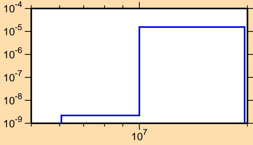
\sigma vs. E for ^{255}\text{Lw}(\text{mt } 45)
