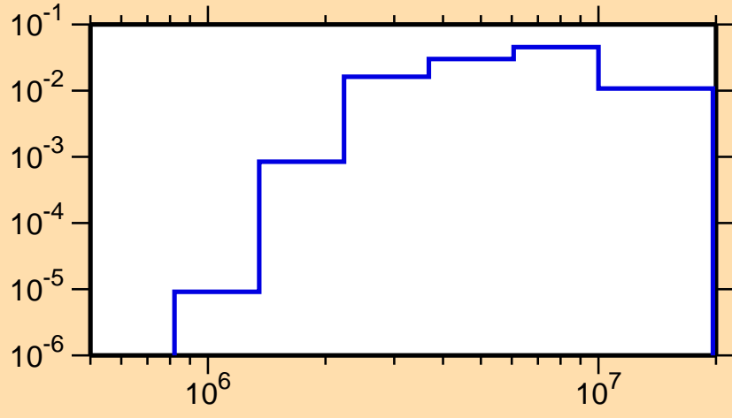
\sigma vs. E for ^{255}\text{Lw}(n,n\alpha)
