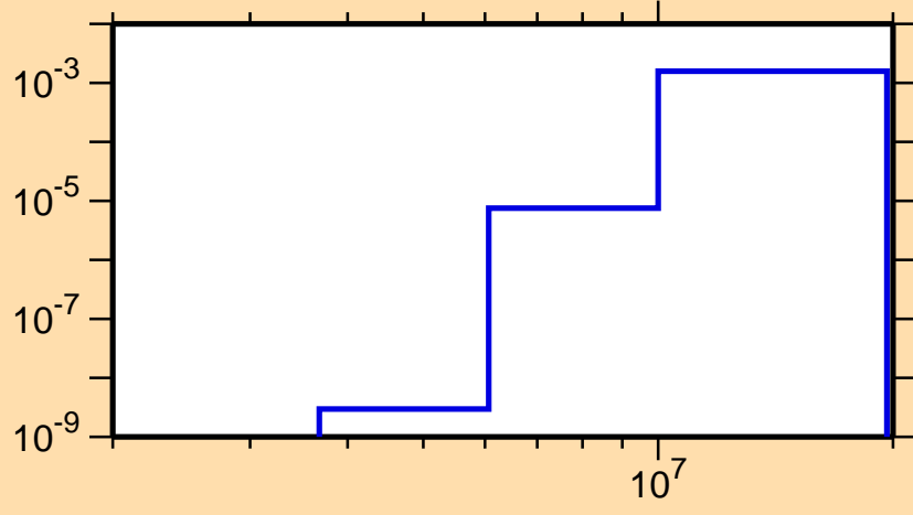
\sigma vs. E for ^{255}\text{Lw}(n,np)
