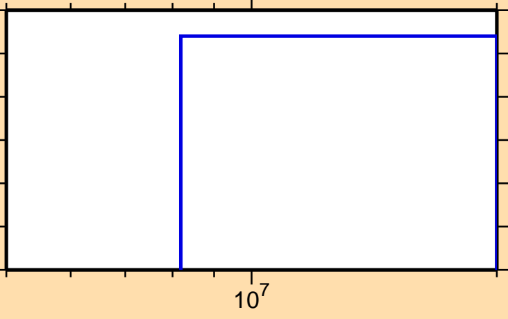
\sigma vs. E for ^{255}\text{Lw}(n,2np)
