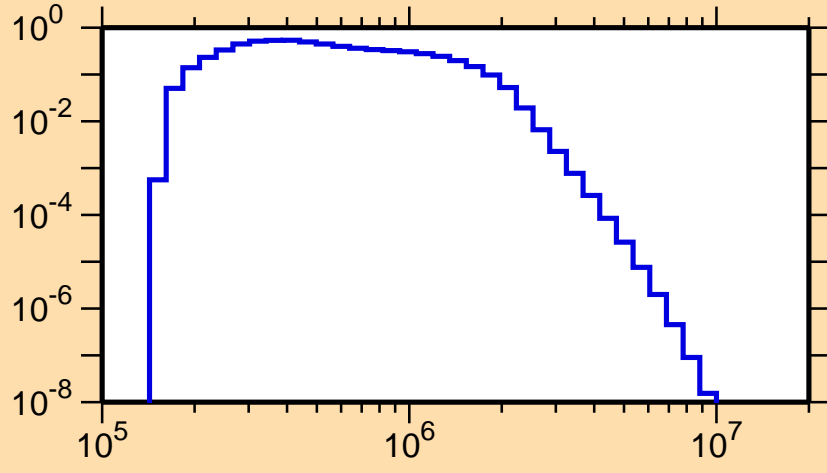
\sigma vs. E for ^{255}\text{Lw}(n,n_2)
