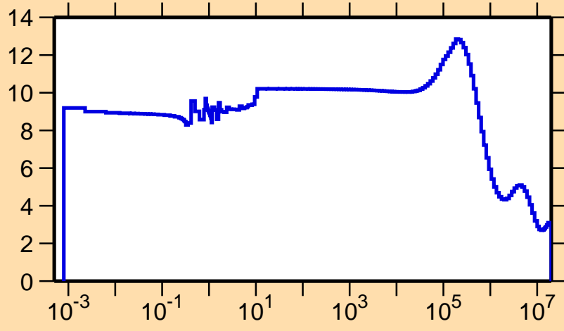
\sigma vs. E for ^{255}\text{Lw}(n,\text{el.})
