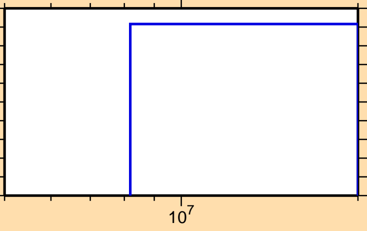
\sigma vs. E for ^{255}\text{Lw}(n,nt)
