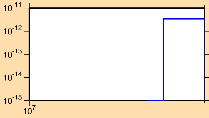
\sigma vs. E for ^{256}\text{Lw} (mt 42)
