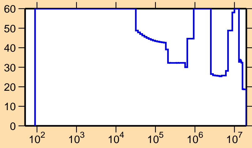
\Delta\sigma/\sigma vs. E for ^{256}\text{Lw}(n,el.)
