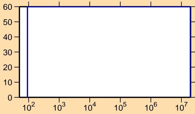
\Delta\sigma/\sigma vs. E for ^{256}\text{Lw}(n,\gamma)
