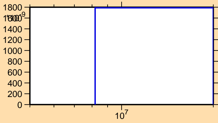
\sigma vs. E for ^{256}\text{Lw}(n,nd)
