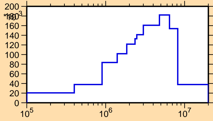
\sigma vs. E for ^{256}\text{Lw}(n,n\alpha)
