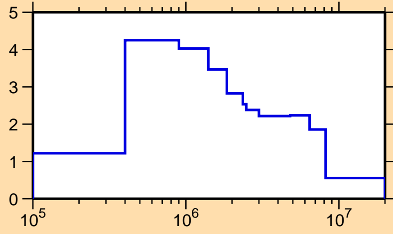
\sigma vs. E for ^{256}\text{Lw}(n,\text{inel.})
