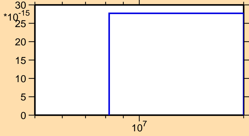
\sigma vs. E for ^{256}\text{Lw}(\text{mt } 42)
