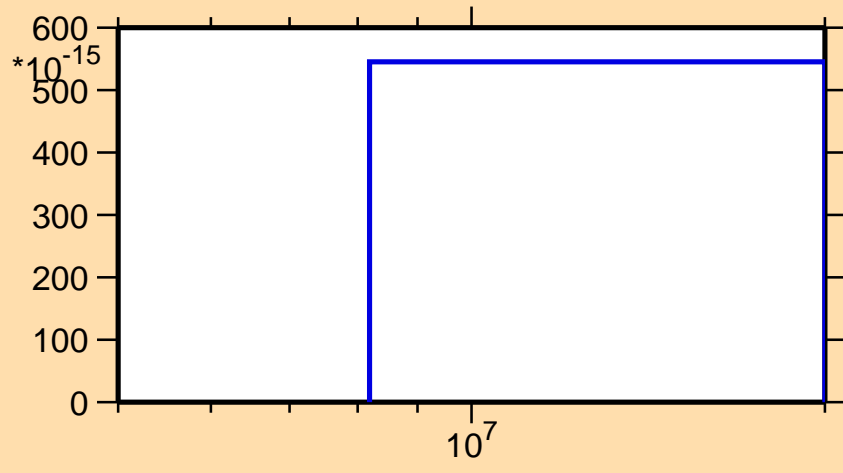
\sigma vs. E for ^{256}\text{Lw}(\text{mt 34})
