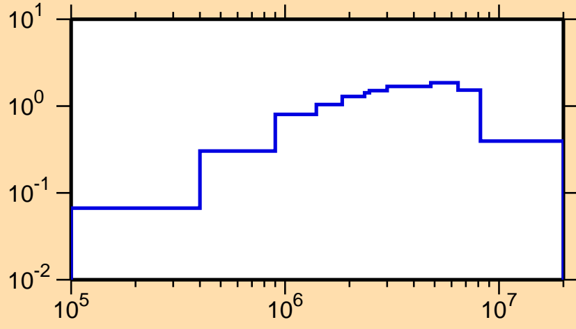
\sigma vs. E for ^{256}\text{Lw}(n,n\text{cont.})
