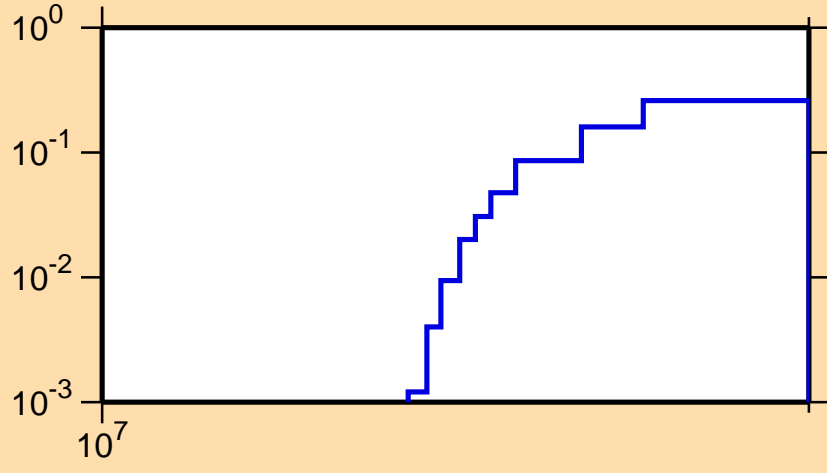
\sigma vs. E for ^{257}\text{Lw}(n,3n)
