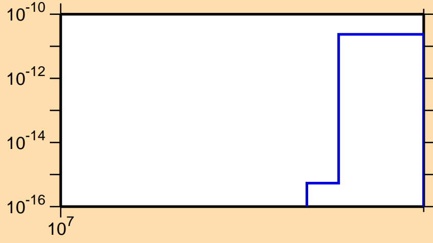
\sigma vs. E for ^{257}\text{Lw} (mt 11)
