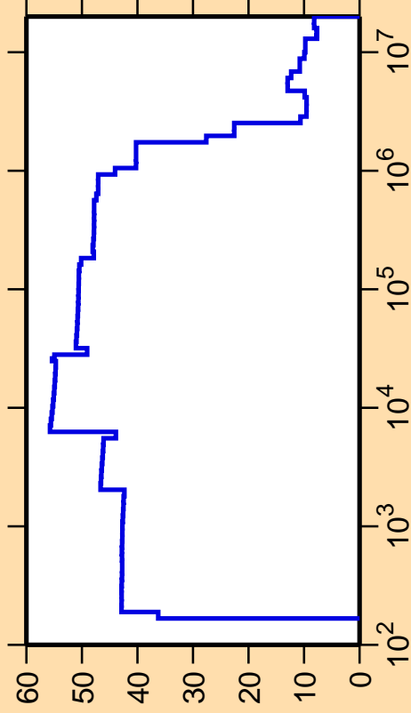
\Delta\sigma/\sigma vs. E for ^{257}\text{Lw}(n,\text{nonel.})
