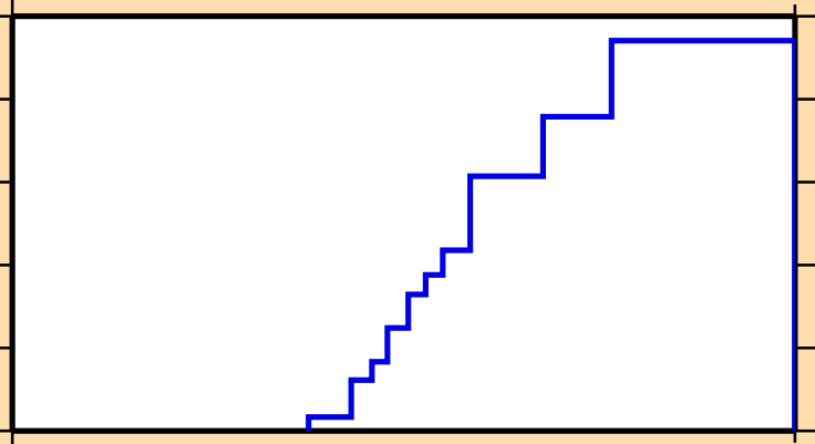
\sigma vs. E for ^{257}\text{Lw}(n,nd)
