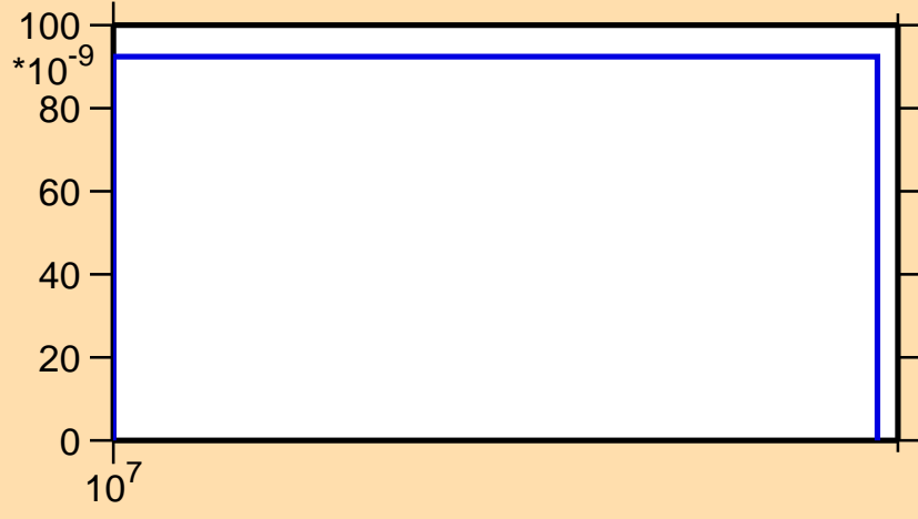
\sigma vs. E for ^{257}\text{Lw}(n,2np)
