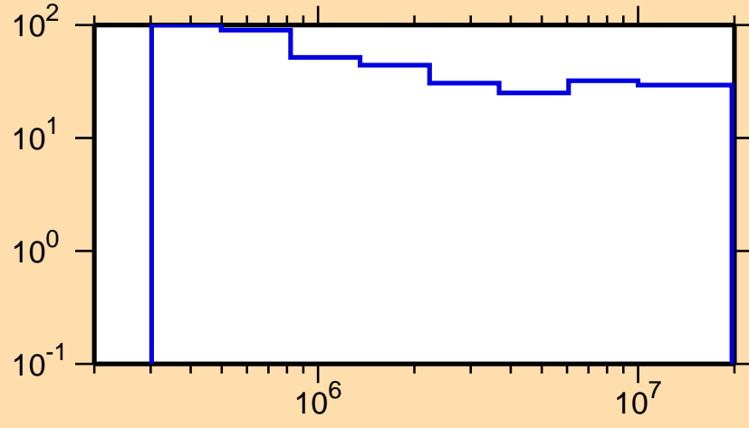
\Delta\sigma/\sigma vs. E for ^{257}\text{Lw}(n,n\text{cont.})
