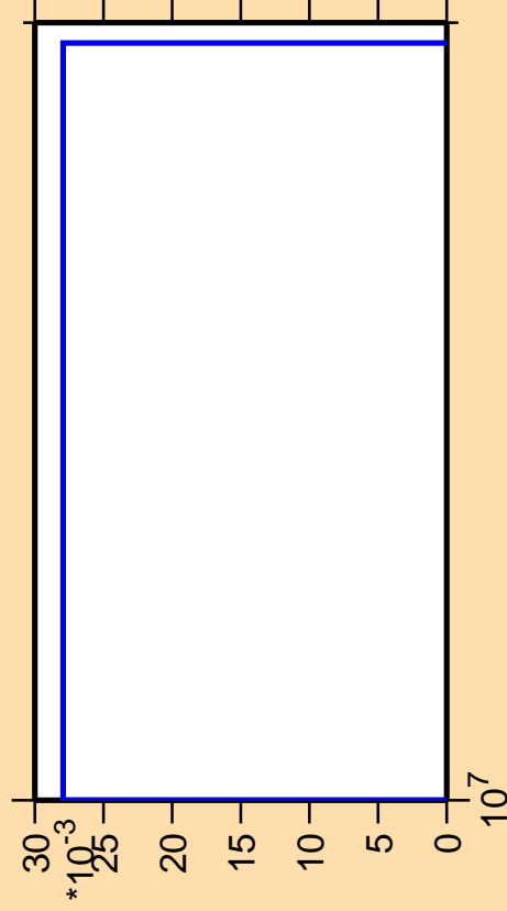
\Delta\sigma/\sigma vs. E for ^{257}\text{Lw} (mt 34)
