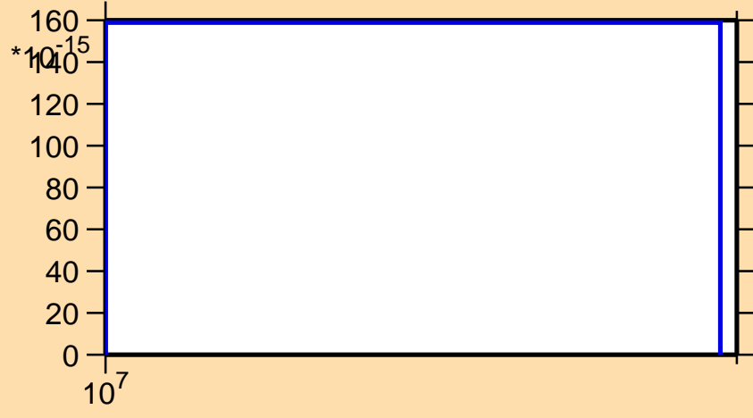
\sigma vs. E for ^{257}\text{Lw}(\text{mt 11})
