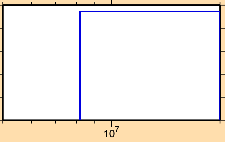
\sigma vs. E for ^{257}\text{Lw}(n,3n\alpha)
