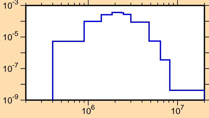
\sigma vs. E for ^{257}\text{Lw}(n,n_4)
