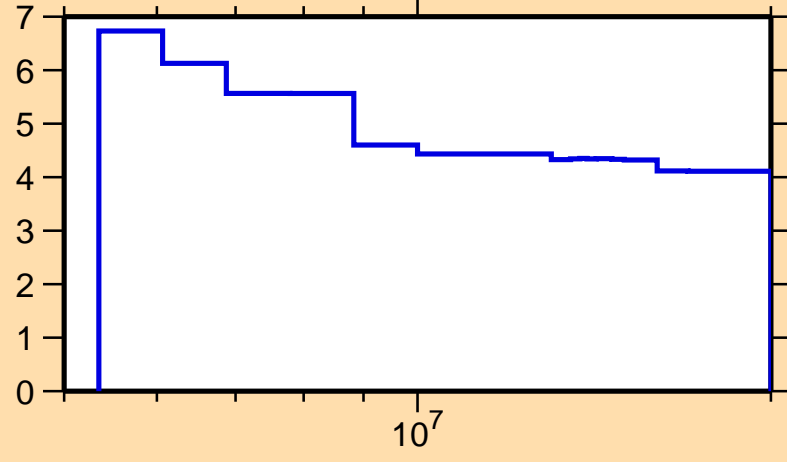
\Delta\sigma/\sigma vs. E for ^{258}\text{Lw}(n,\text{nonel.})
