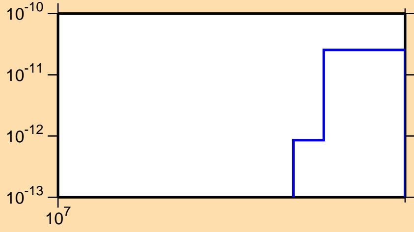
\sigma vs. E for ^{258}\text{Lw} (mt 34)
