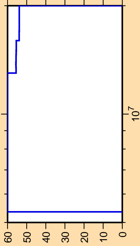
\Delta\sigma/\sigma vs. E for ^{258}\text{Lw}(n,\alpha)
