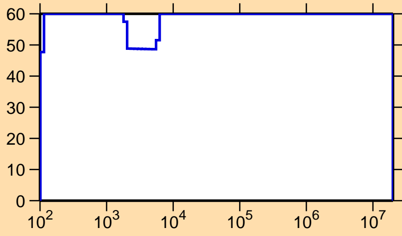
\Delta\sigma/\sigma vs. E for ^{258}\text{Lw}(n,\gamma)
