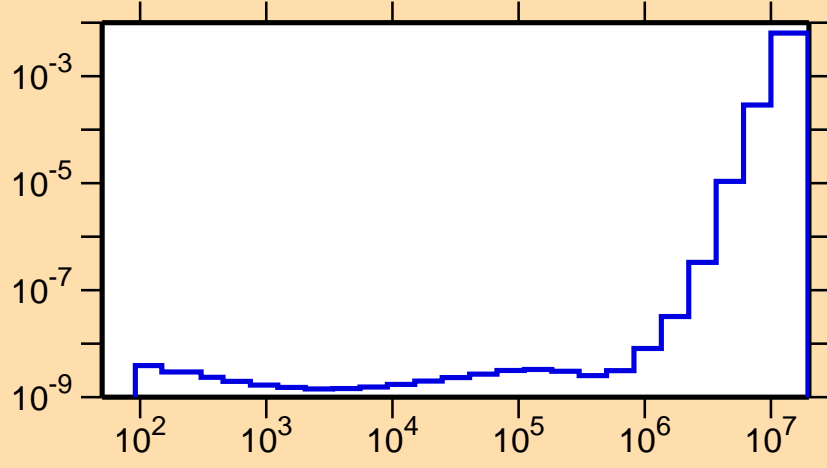
\sigma vs. E for ^{258}\text{Lw}(n,p\alpha)
