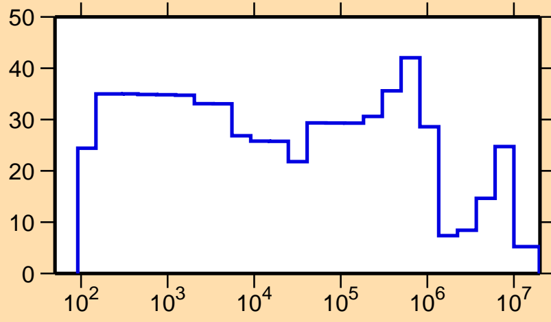
\Delta\sigma/\sigma vs. E for ^{258}\text{Lw}(n,\text{el.})
