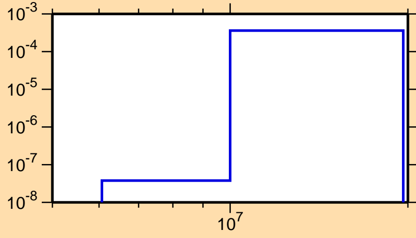
\sigma vs. E for ^{258}\text{Lw}(n,d)
