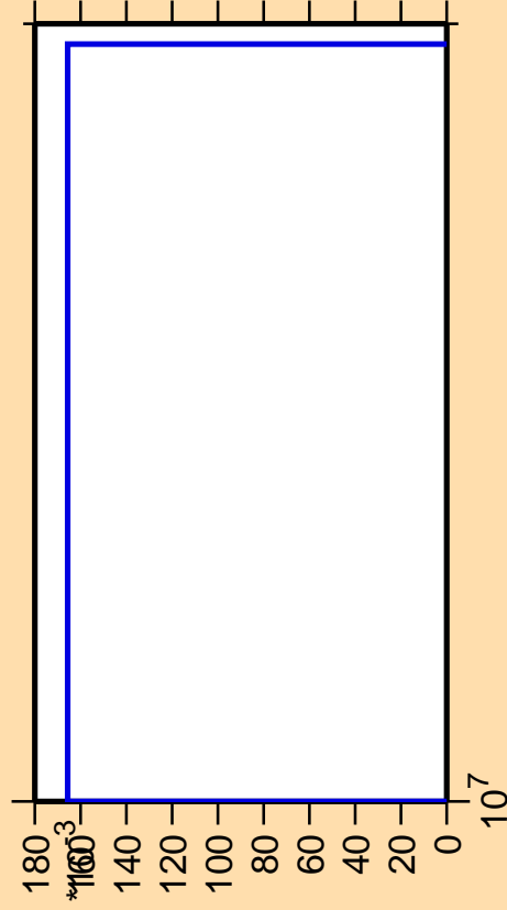
\Delta\sigma/\sigma vs. E for ^{258}\text{Lw} (mt 34)
