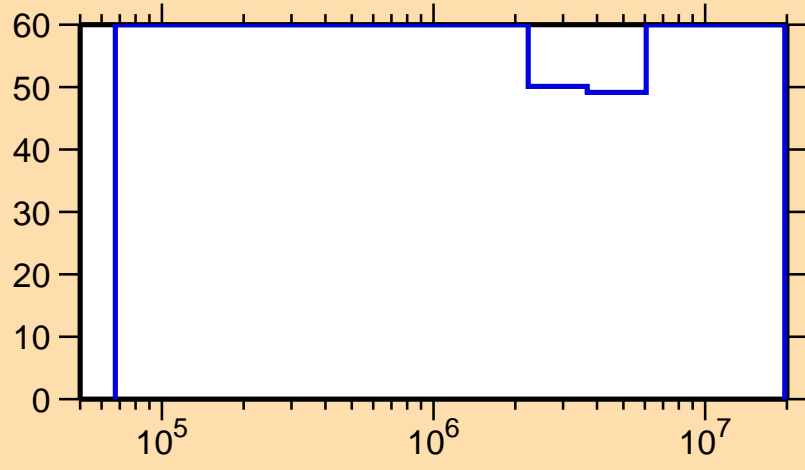
\Delta\sigma/\sigma vs. E for ^{258}\text{Lw}(n,n\text{cont.})
